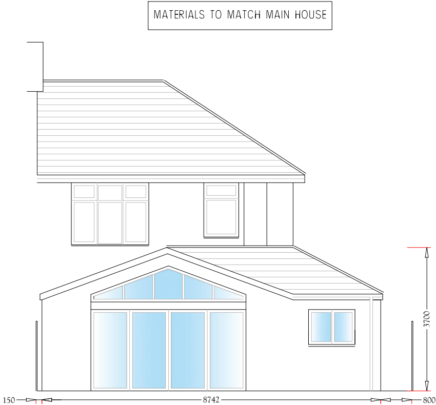
rear SOUTH – WEST elevation
