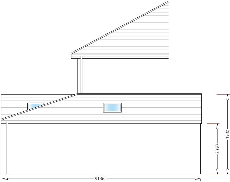
side SOUTH – EAST elevation
