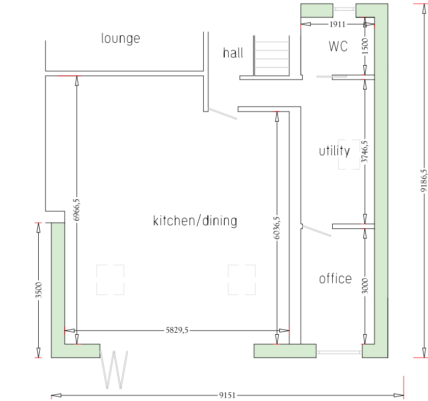
Ground Floor Plan (Part)
