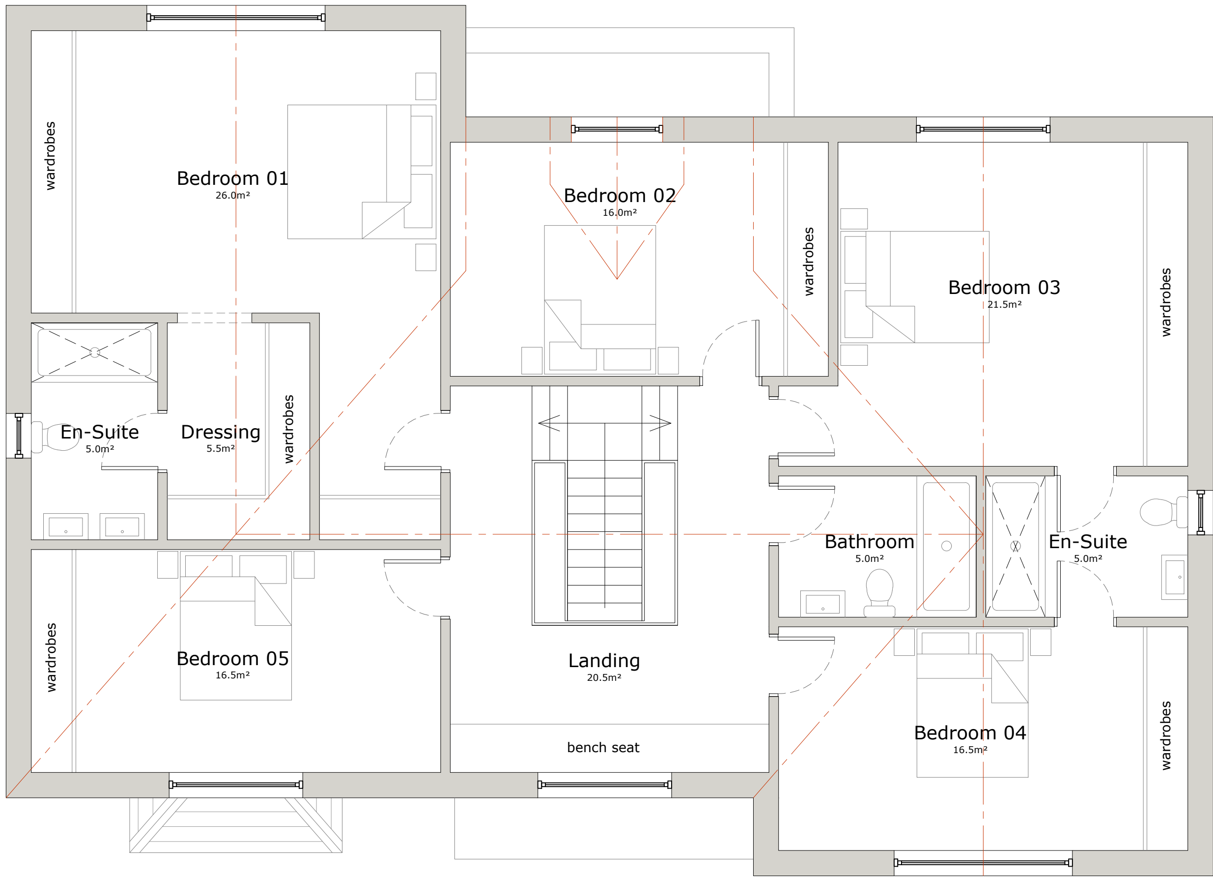
First Floor 144.0m 2
