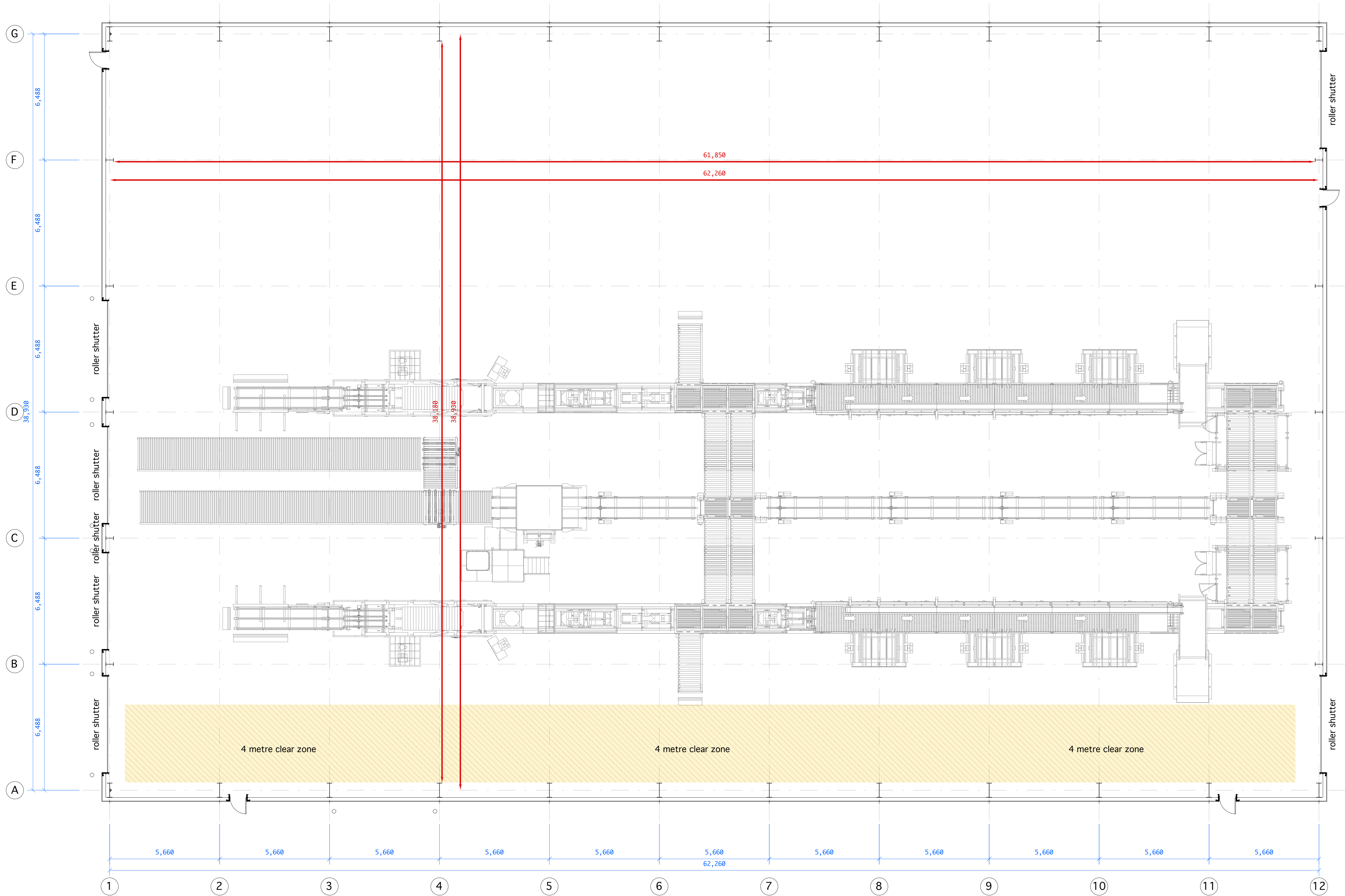
GROUND FLOOR
