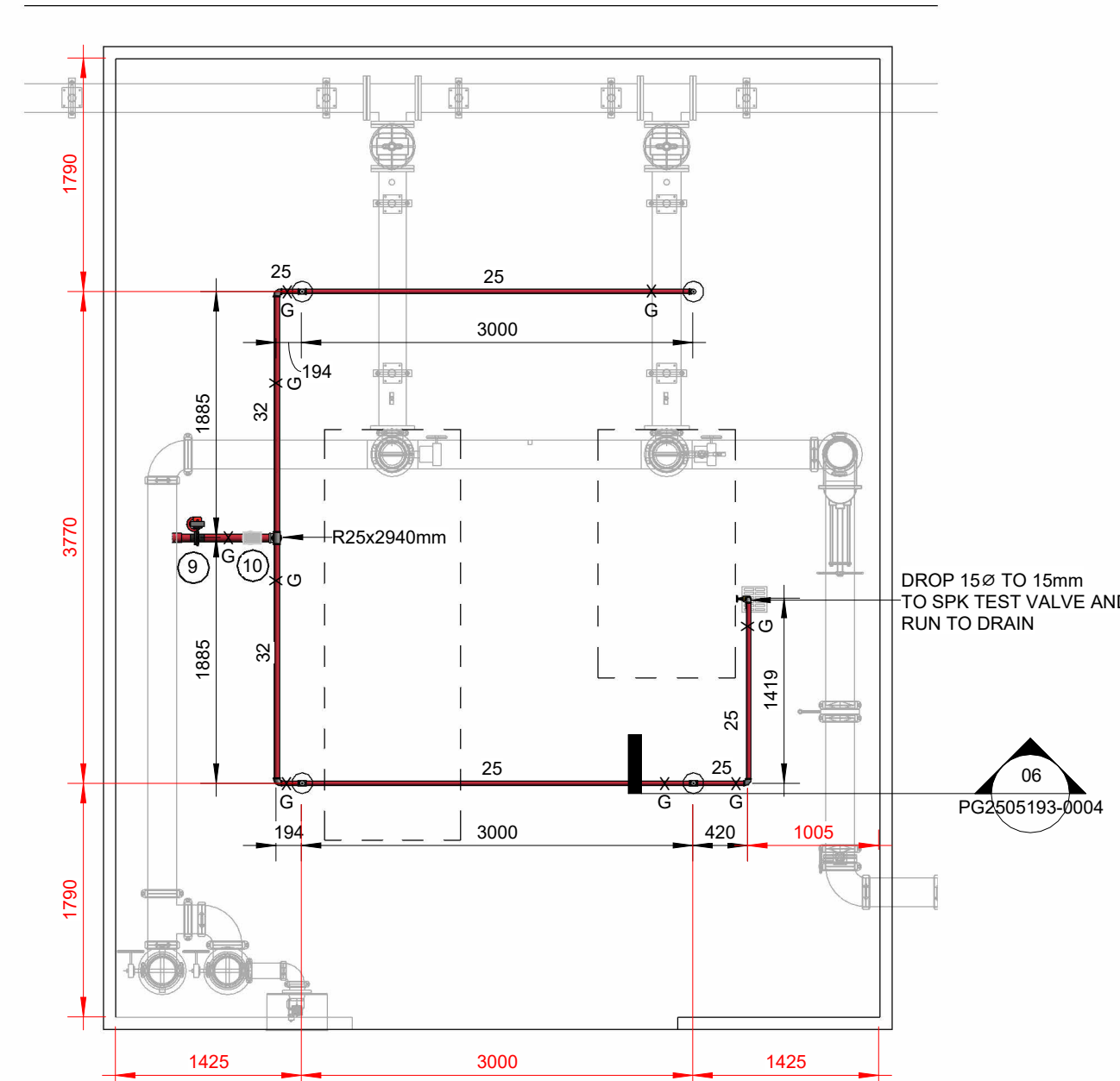
04 PUMPHOUSE SPK PROTECTION
