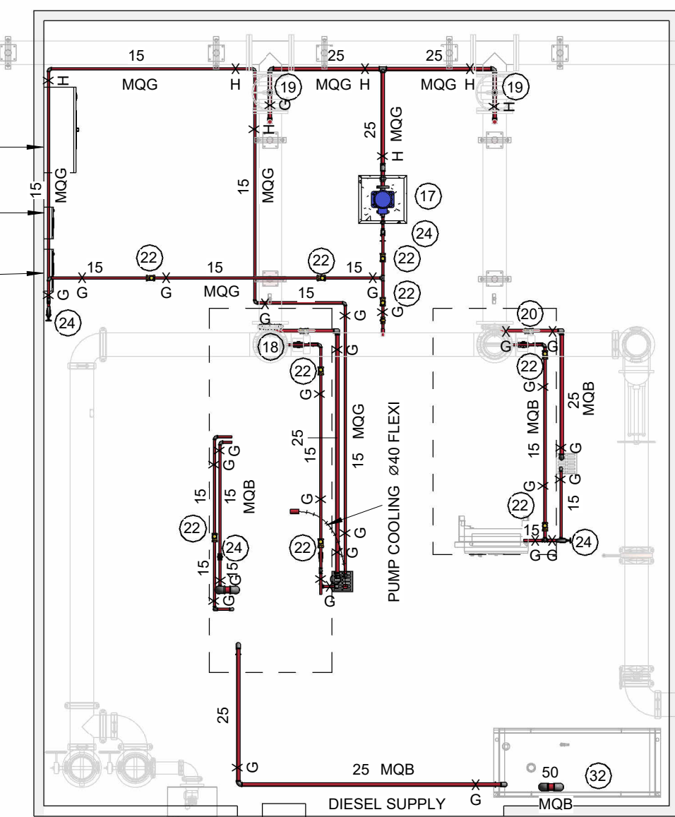
03 PLAN OF TRIM PIPEWORK
