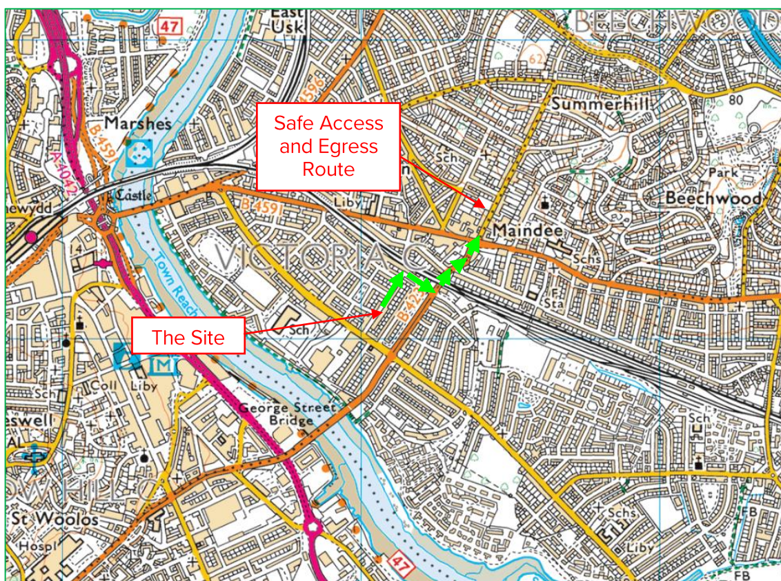
Figure 15 - Safe Access and Egress Route
