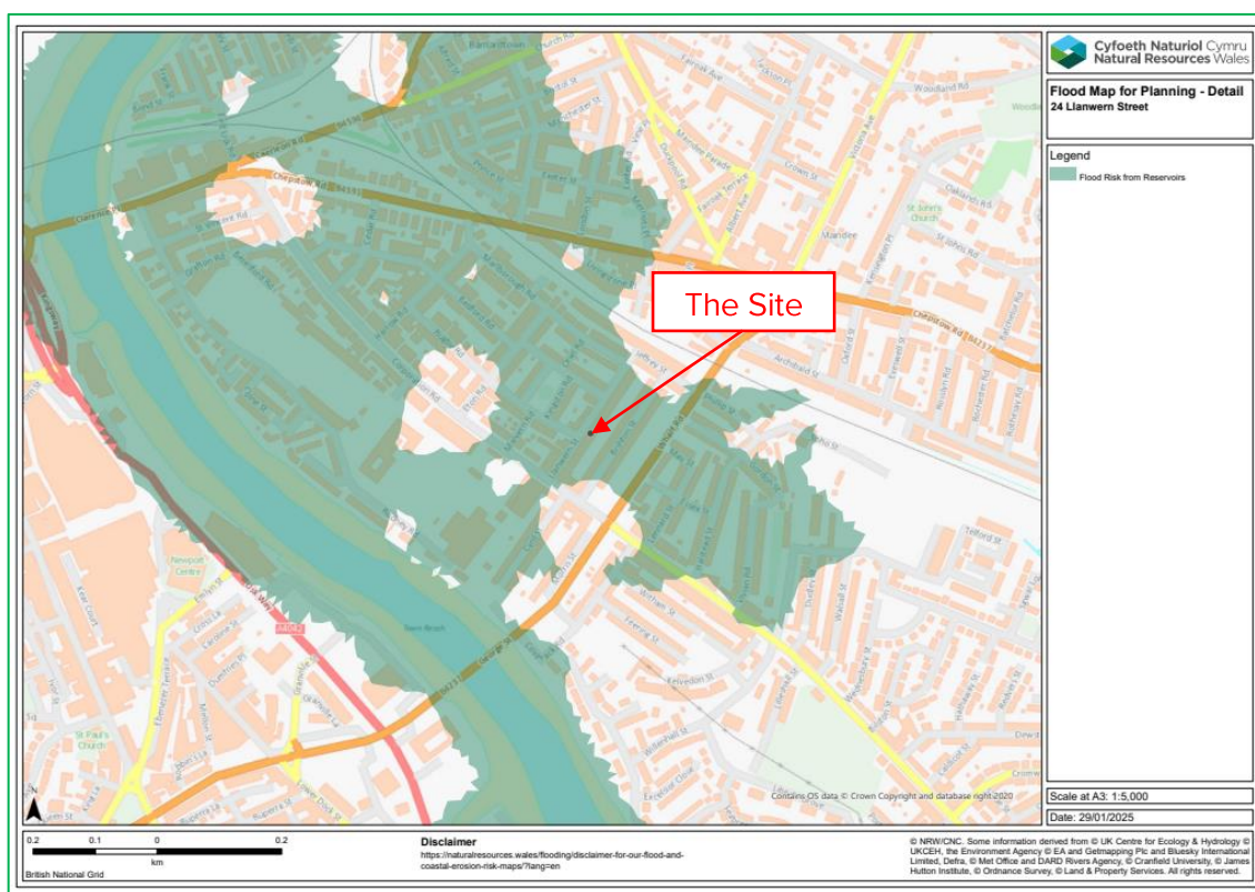
Figure 14 - Natural Resources Wales Reservoir Flood Map
