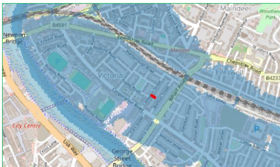
Figure 12 - Natural Resources Wales Breach Modelled 1 in 200 Year in 2115 Flood Outline
