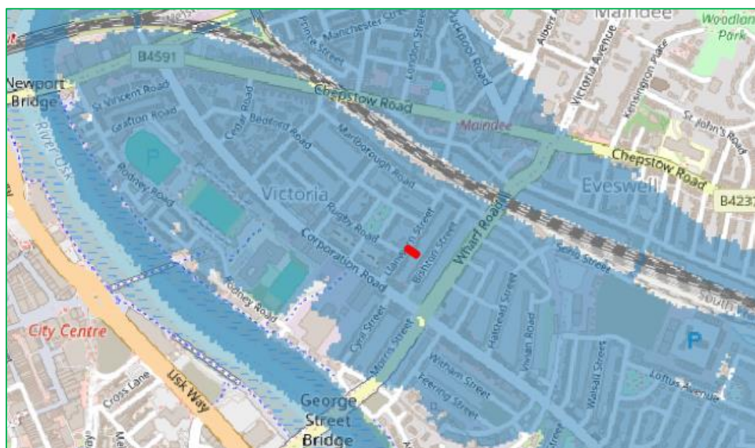
Figure 9 - Natural Resources Wales Undefended Modelled 1 in 1000 Year Flood Outline
