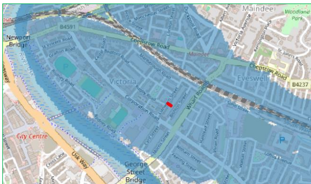
Figure 7 - Natural Resources Wales Defended Modelled 1 in 1000 Year in 2115 Flood Outline
