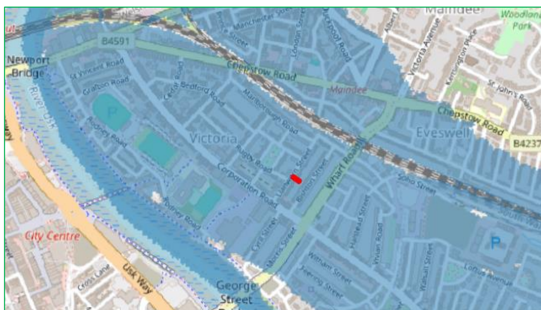
Figure 13 - Natural Resources Wales Breach Modelled 1 in 1000 Year in 2115 Flood Outline
