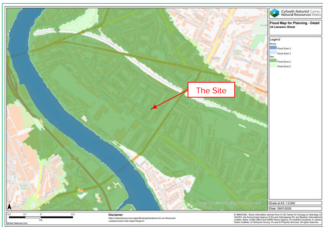
Figure 3 - Flood Map for Planning: Rivers and Sea
