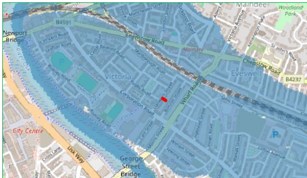
Figure 10 - Natural Resources Wales Undefended Modelled 1 in 200 Year in 2115 Flood Outline
