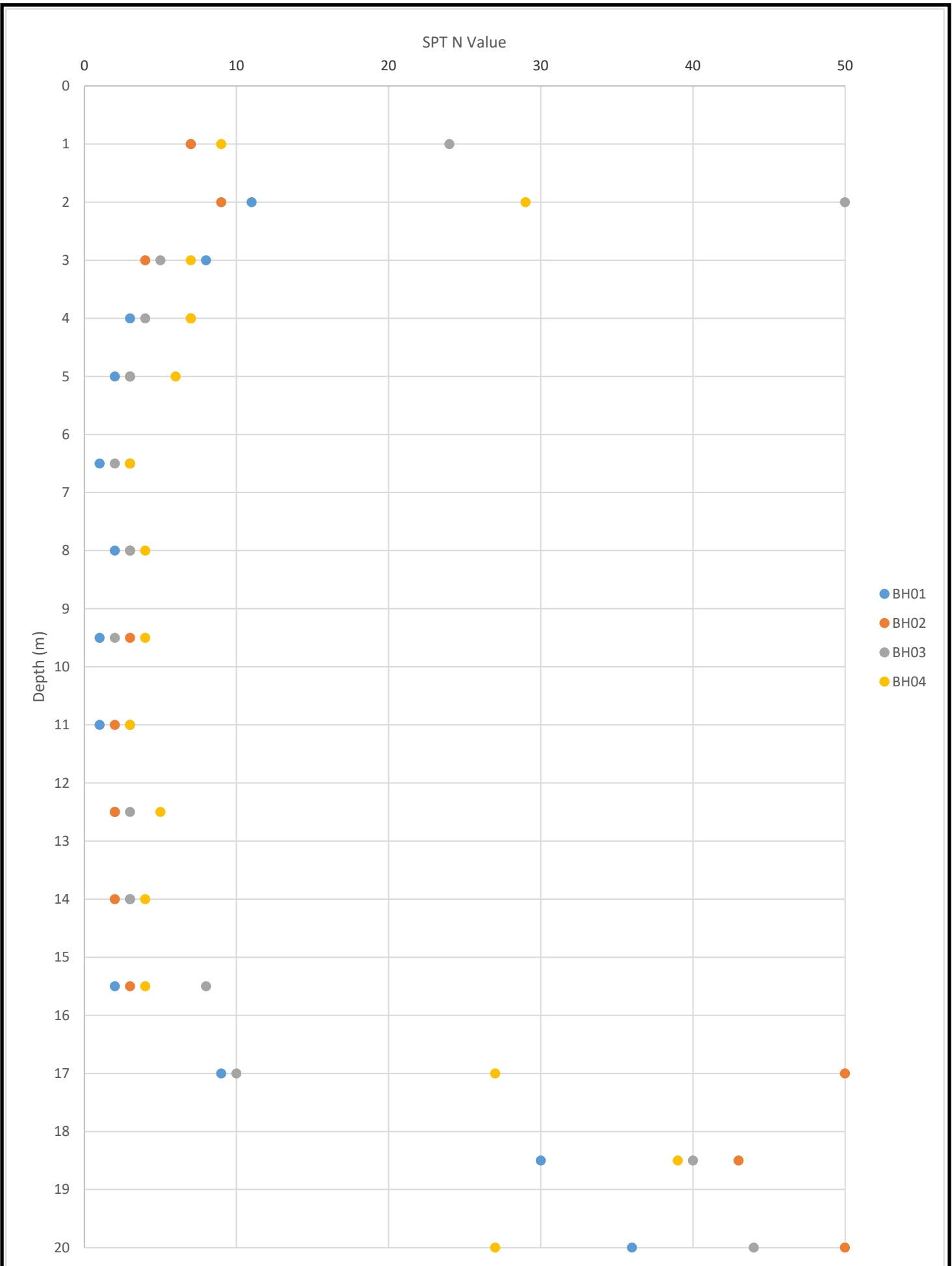
FIGURE 4 - SPT N Value v Depth Plot
