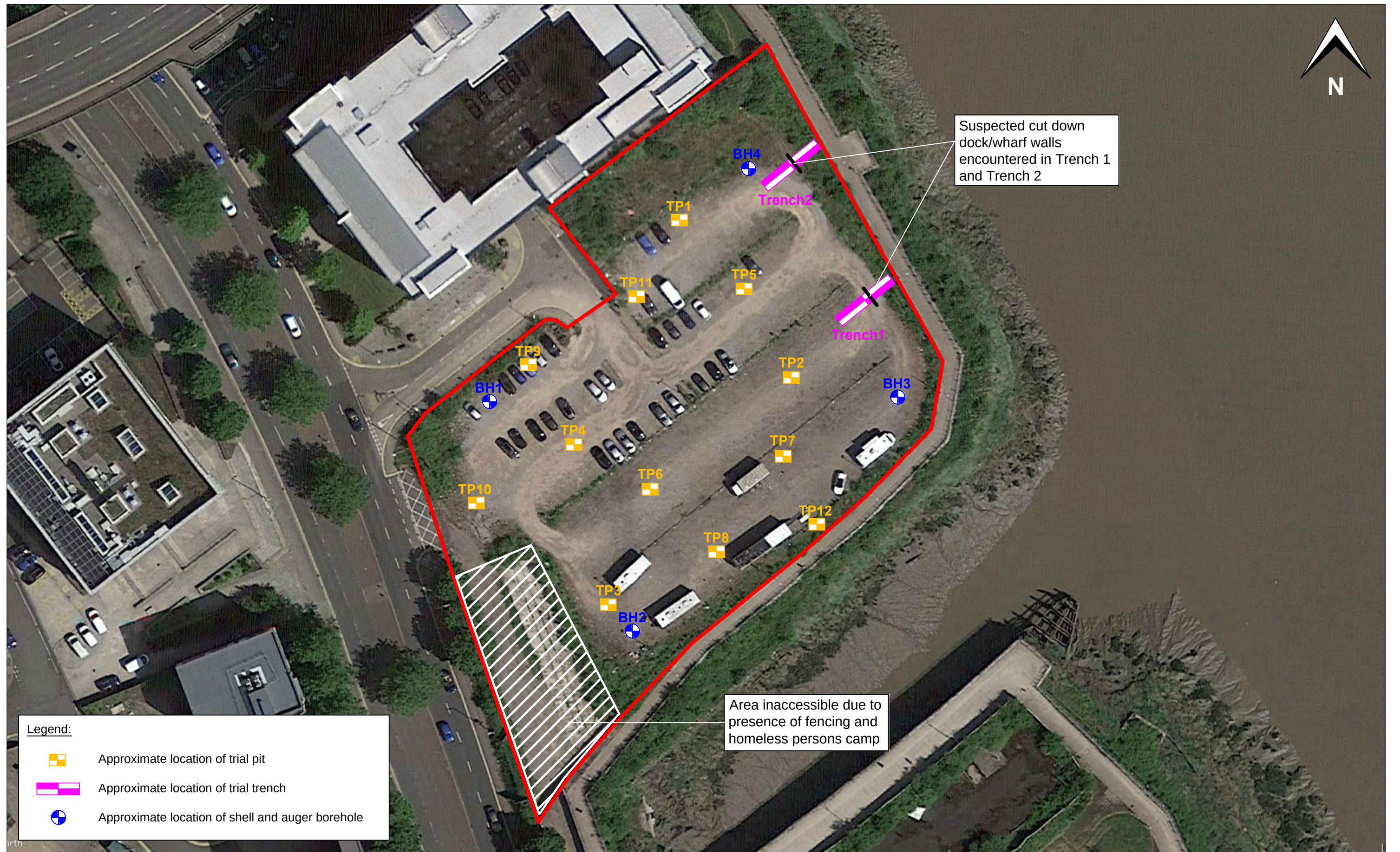
Figure 3: Exploratory Hole Location Plan
