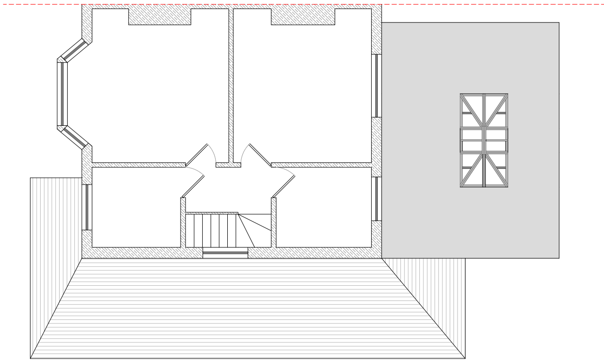
Plan : FIRST FLOOR
