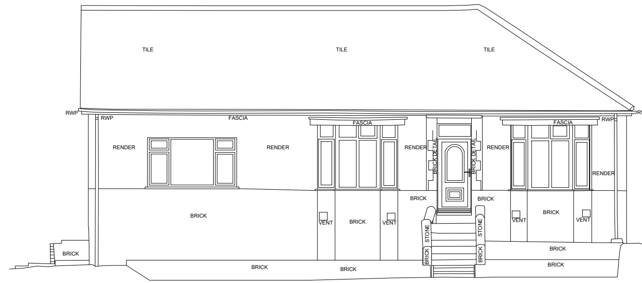
EXISTING SOUTH ELEVATION 1 : 100
