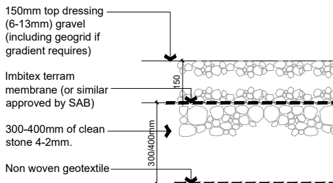
Permeable gravel hard stand
