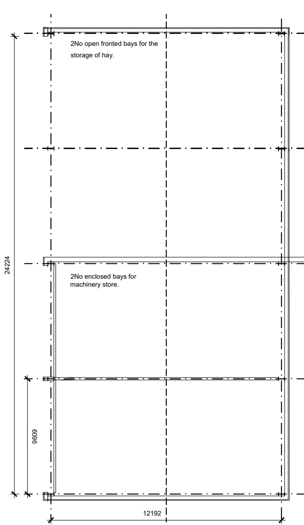
Proposed Floor Plan 1:100 Scale
