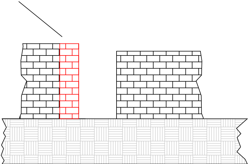
Proposed Elevation 1:50
