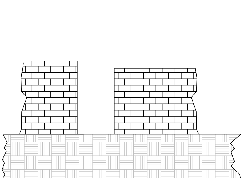
Existing Elevation 1:50
