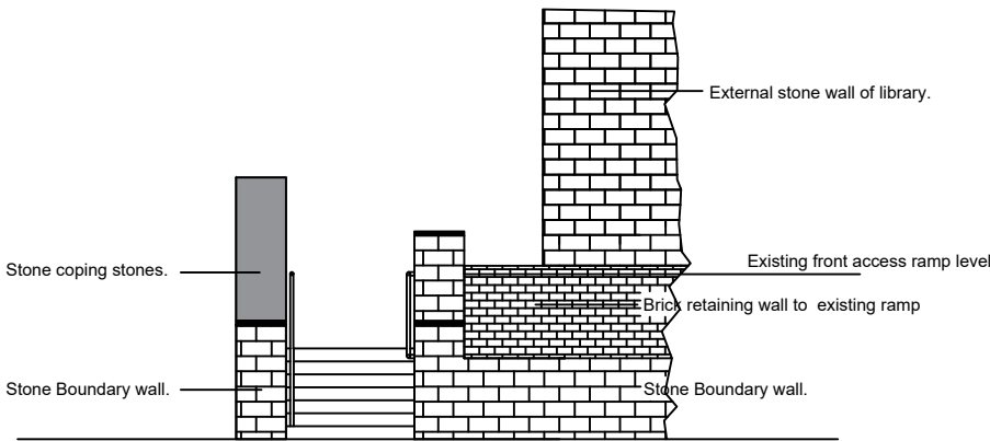
Existing Front Elevation 1:100
