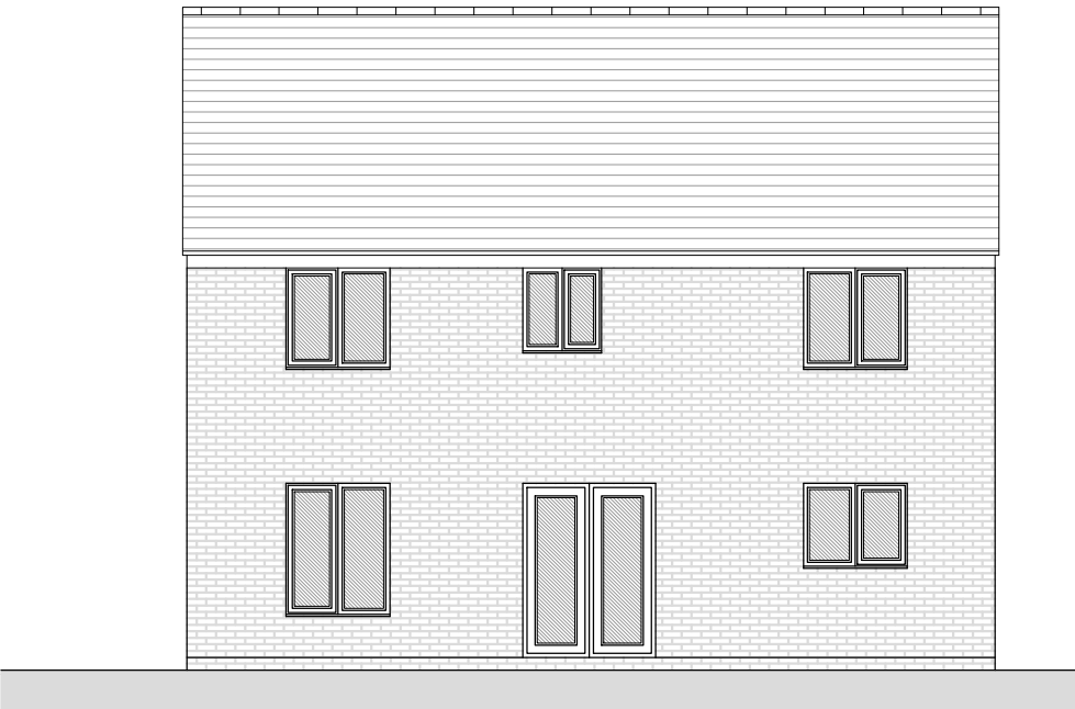
EXISTING REAR ELEVATION 1:100 @ A3
