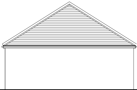
South Elevation as proposed 1:100 scale
