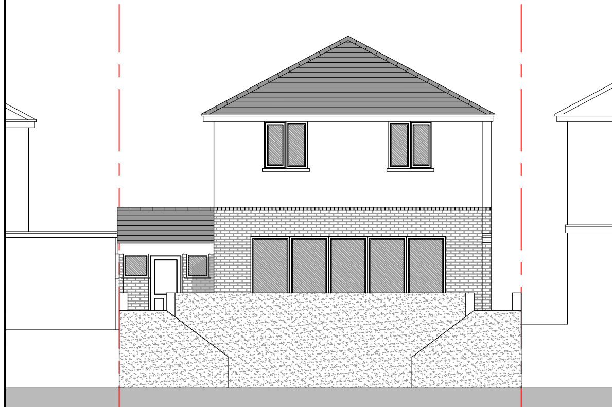
PROPOSED REAR ELEVATION 1:100 @ A3
