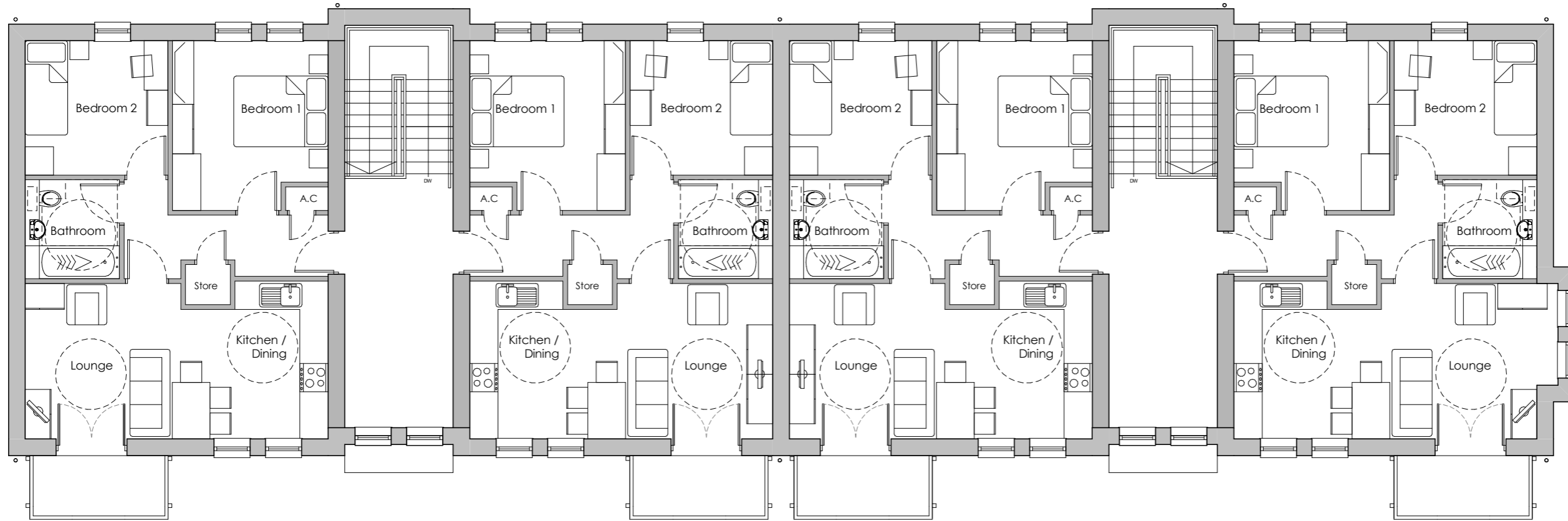
Second Floor Plan House Type 'L1'
