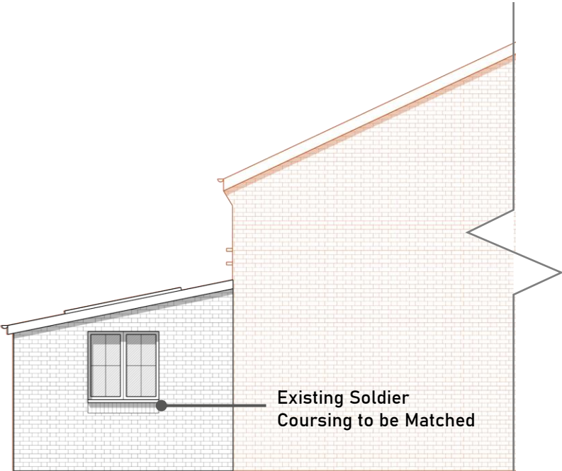
NORTHWEST ELEVATION GA
