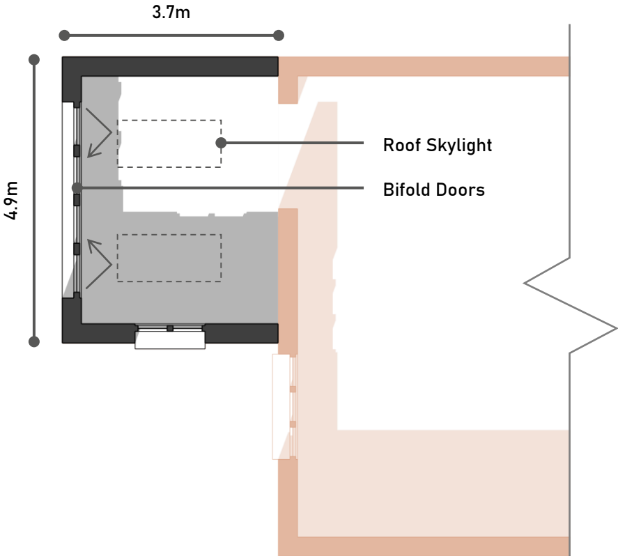
GROUND FLOOR PLAN GA
