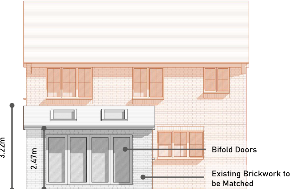
SOUTHWEST ELEVATION GA
