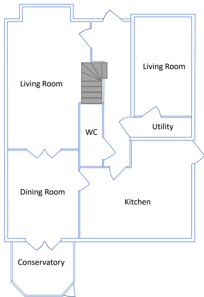
GROUND FLOOR PLAN EXISTING (DRAWN TO SCALE)
