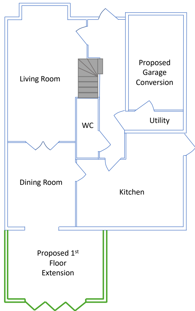
GROUND FLOOR PLAN PROPOSED (DRAWN TO SCALE)
