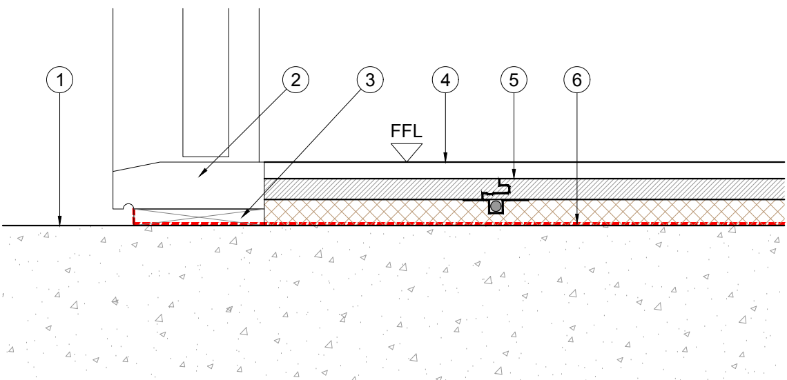
Floor Detail 03:
