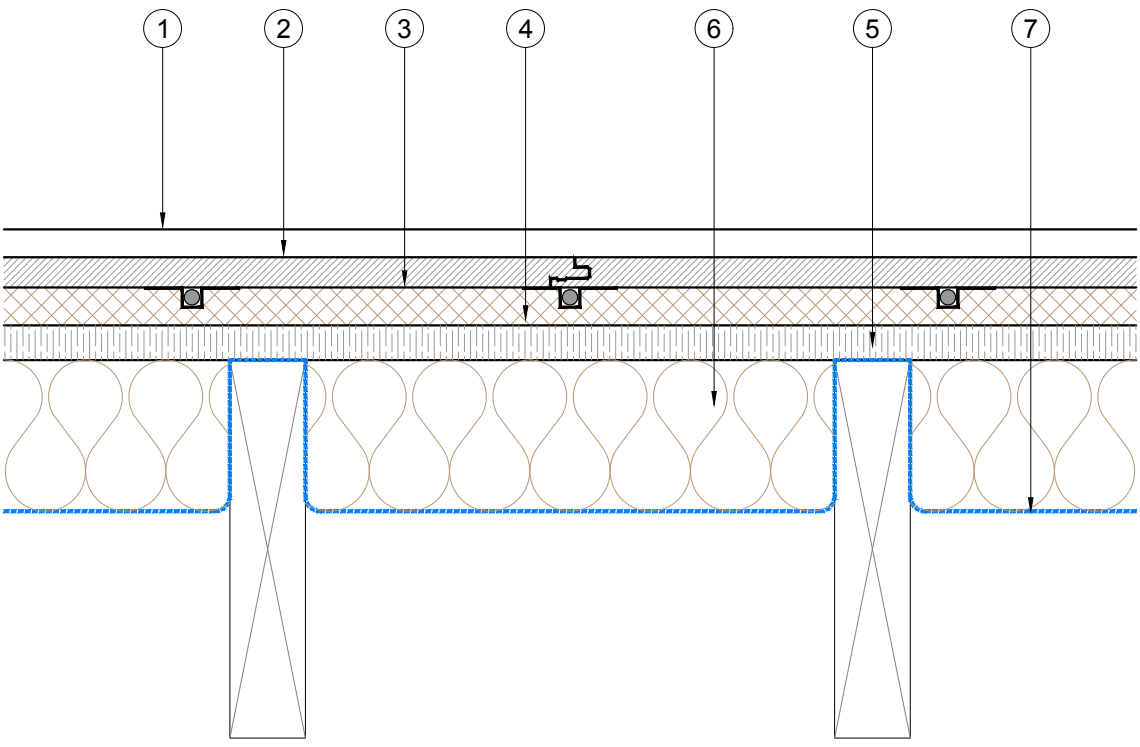
Existing suspended ground floor with thermal upgrade and UFH 1:5
