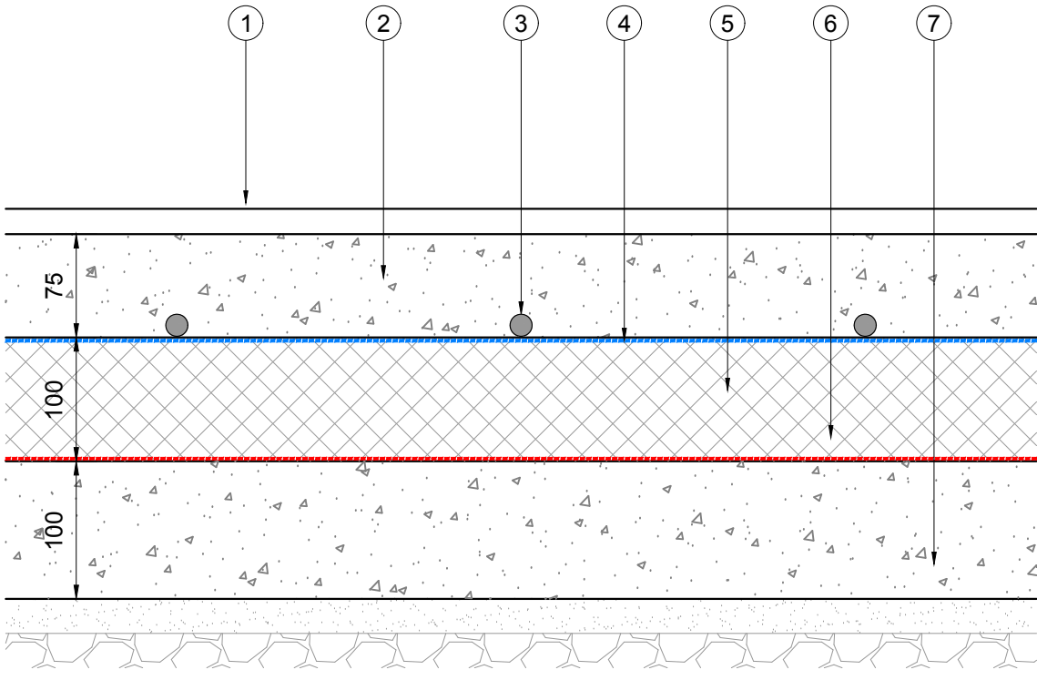
Proposed ground floor build up with UFH 1:5
