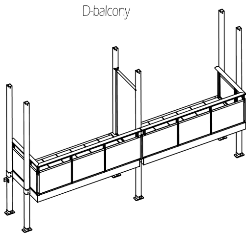
Image 3: 2d dwg ALU 1 double balcony with glazed privacy screen
