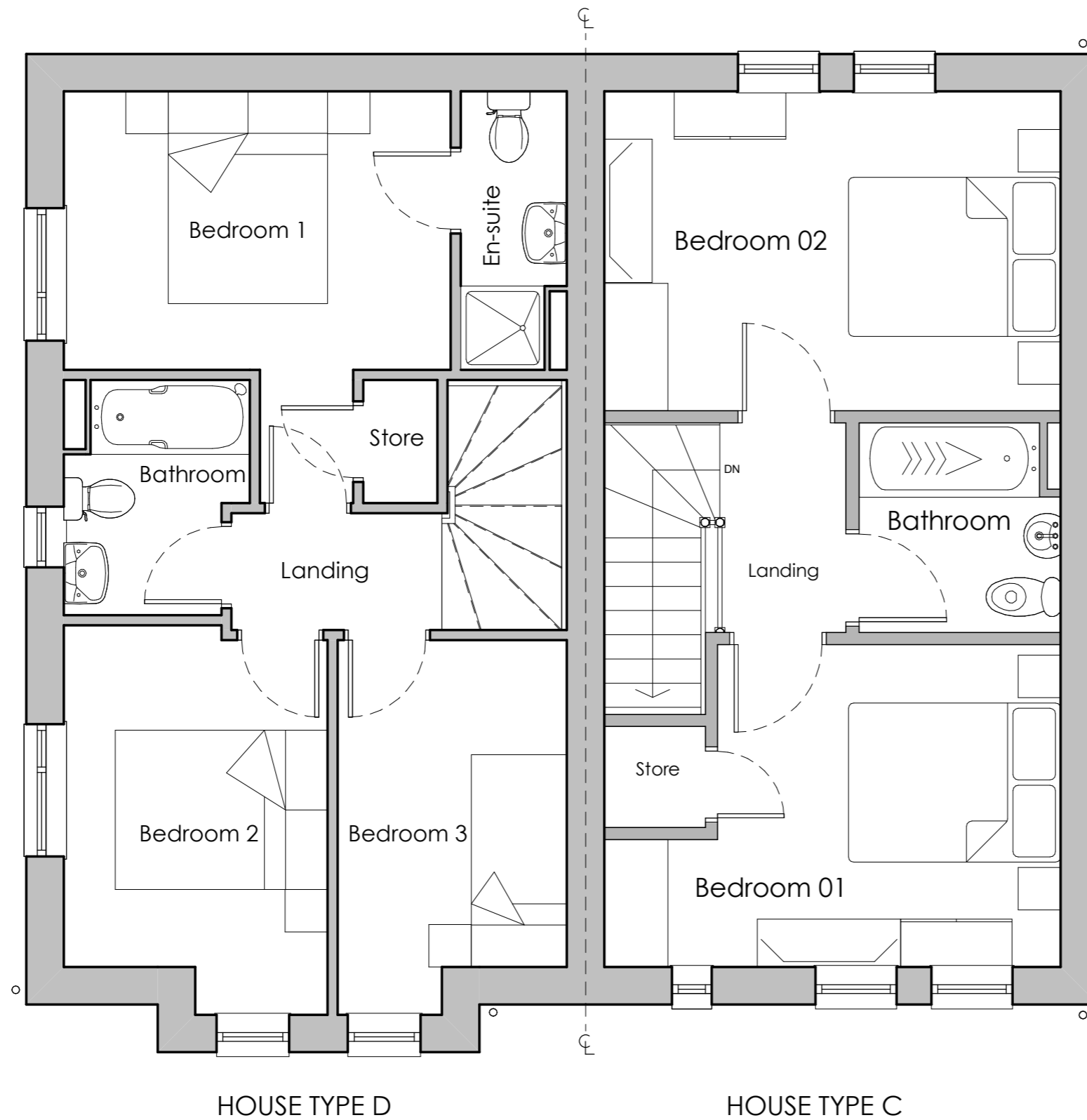
First Floor 1 : 50
