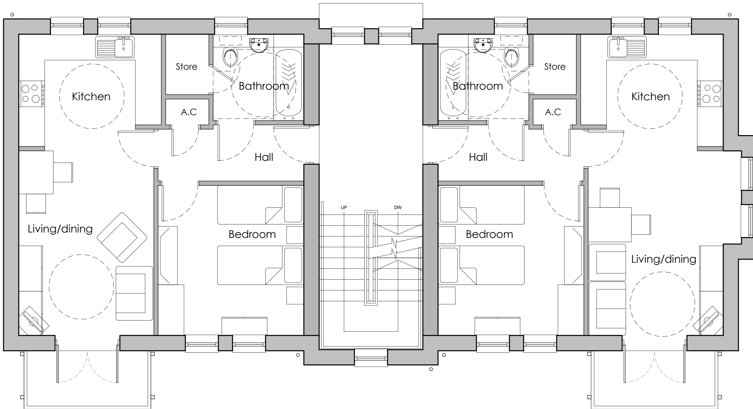
First Floor Plan House Type 'K'
