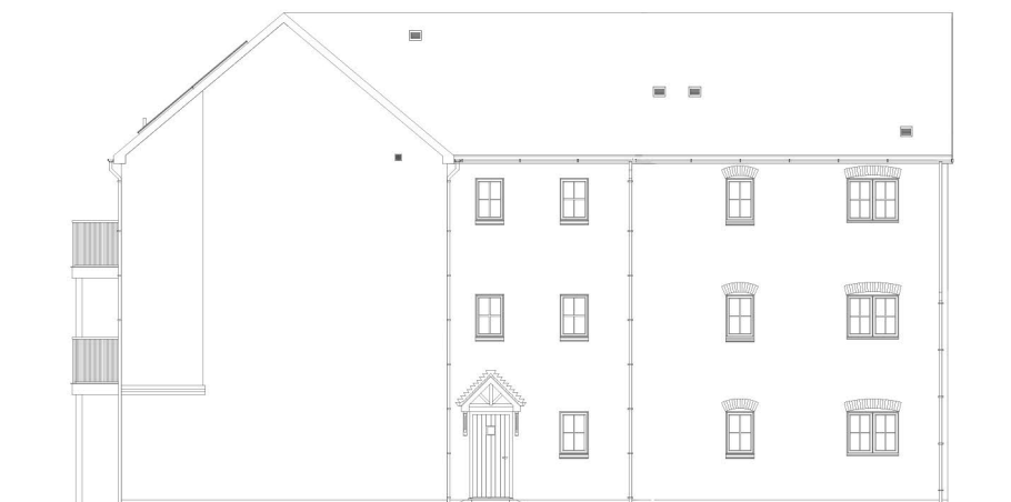
REAR ELEVATION
