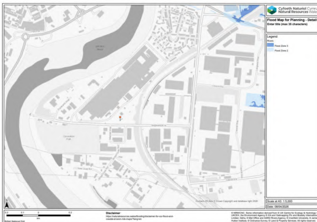
Figure 4.1 Flood map for planning: rivers.
