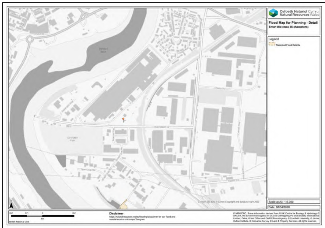
Figure 4.4 Natural Resources Wales historic flood map.
