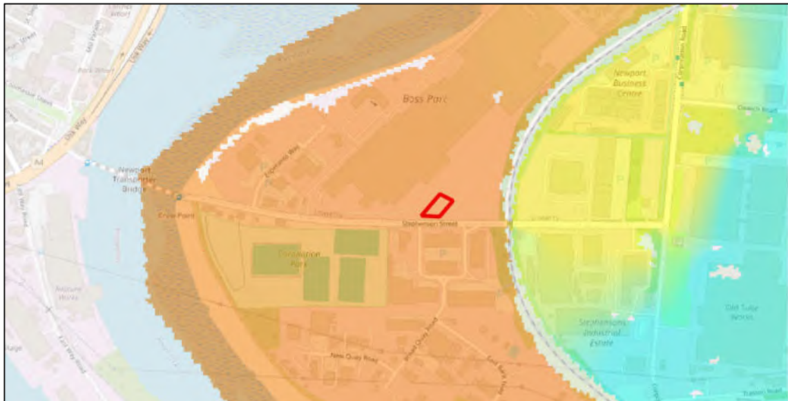
Figure 4.17 Natural Resources Wales breach modelled 1 in 1000 year in 2115 flood outline.
