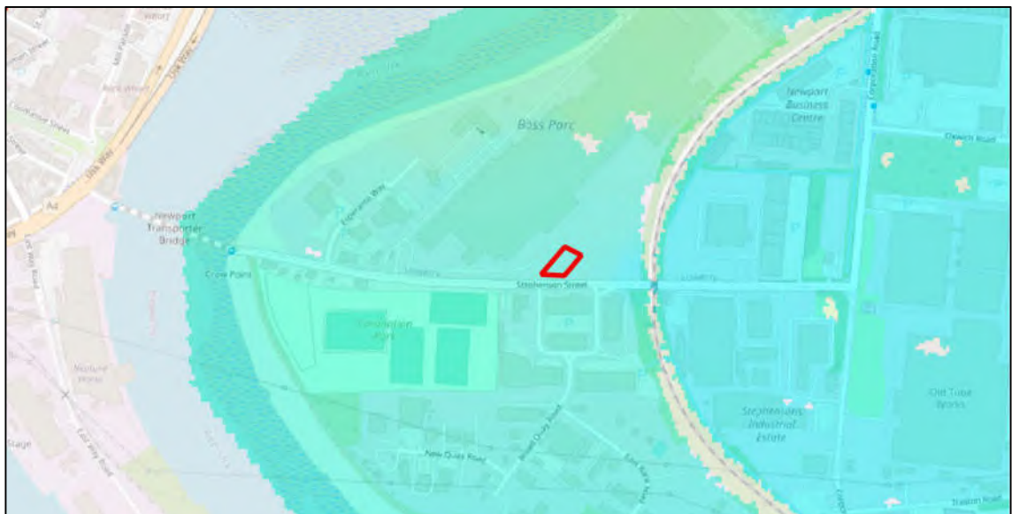
Figure 4.11 Natural Resources Wales undefended modelled 1 in 1000 year flood outline.
