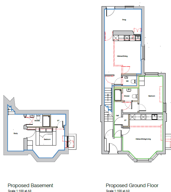
Proposed Plans 1
