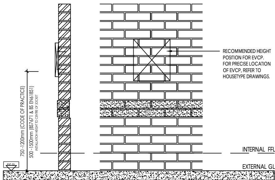
WALL MOUNTED EVCP LOCATION SCALE 1:20
