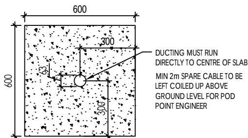
FREE-STANDING MOUNT SLAB DETAIL SCALE 1:20
