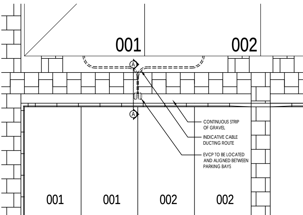
FREE-STANDING MOUNT LOCATION PLAN SCALE 1:100
