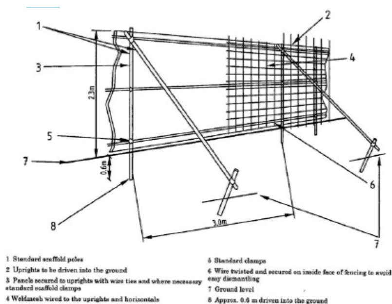
Figure 2 — Protective barrier
