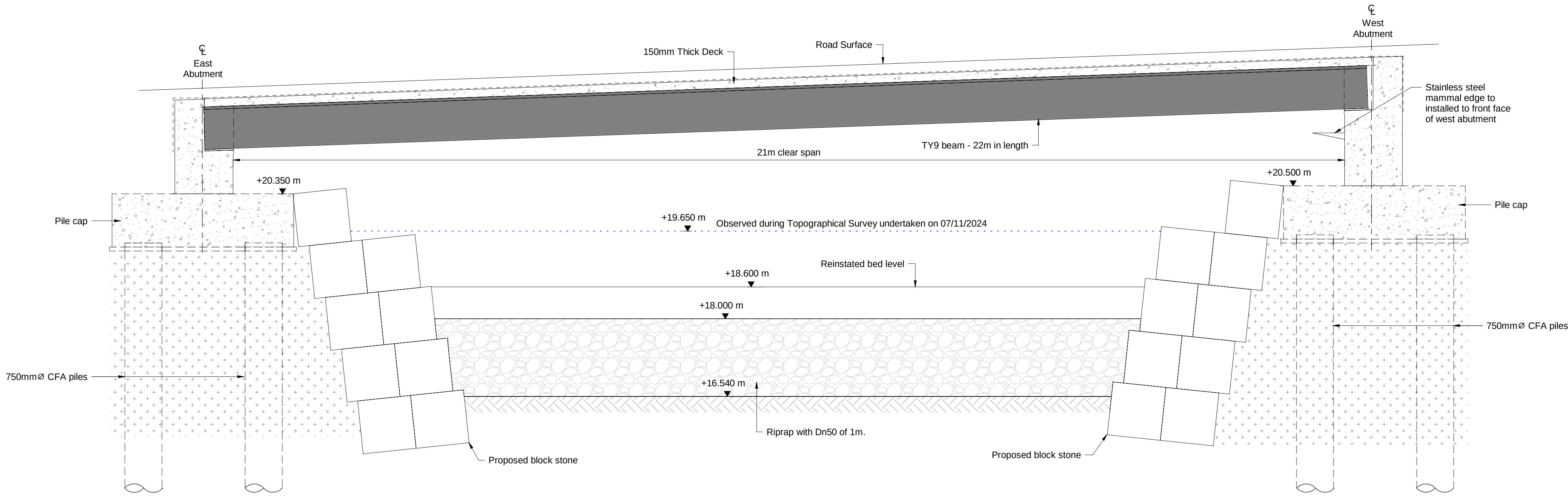
Proposed Cross Section D SCALE 1 : 50
