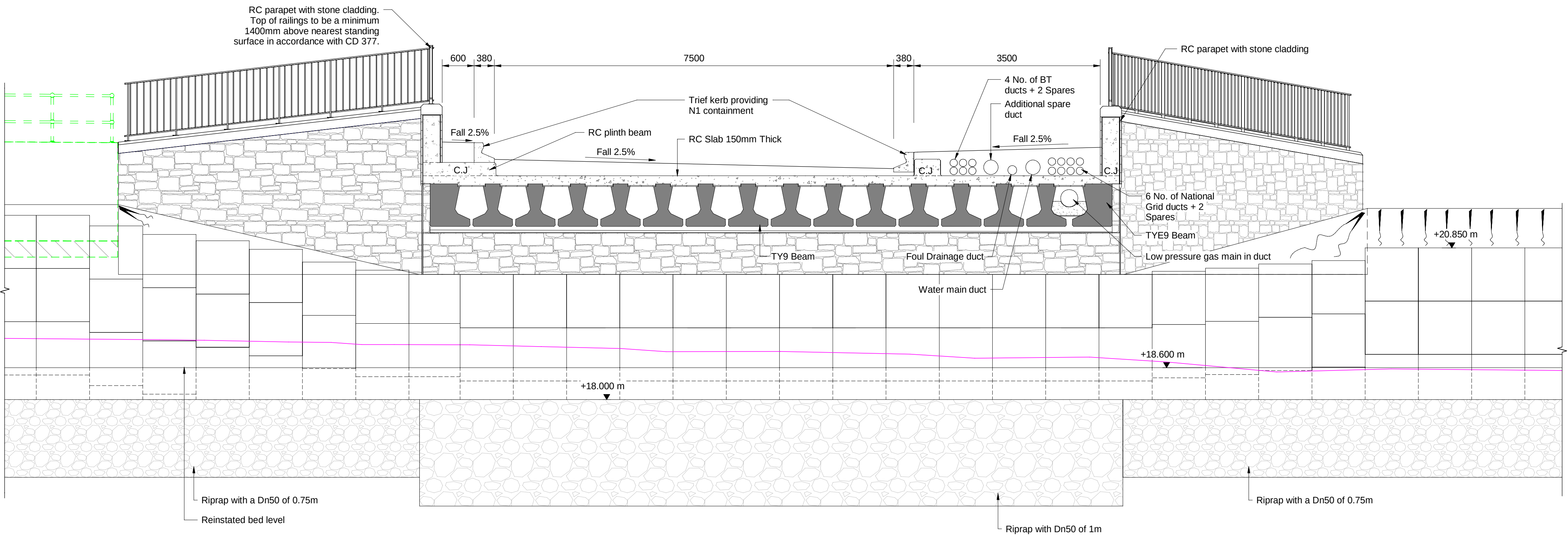
Proposed Section C SCALE 1 : 50
