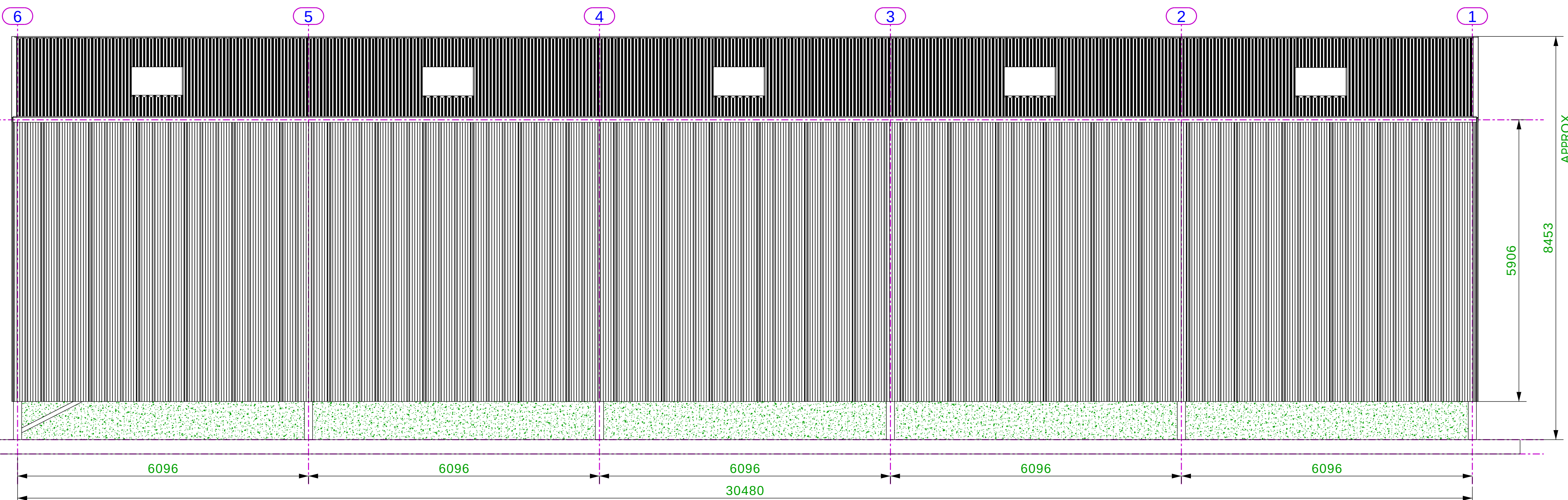
ELEVATION ON GRIDLINE A
