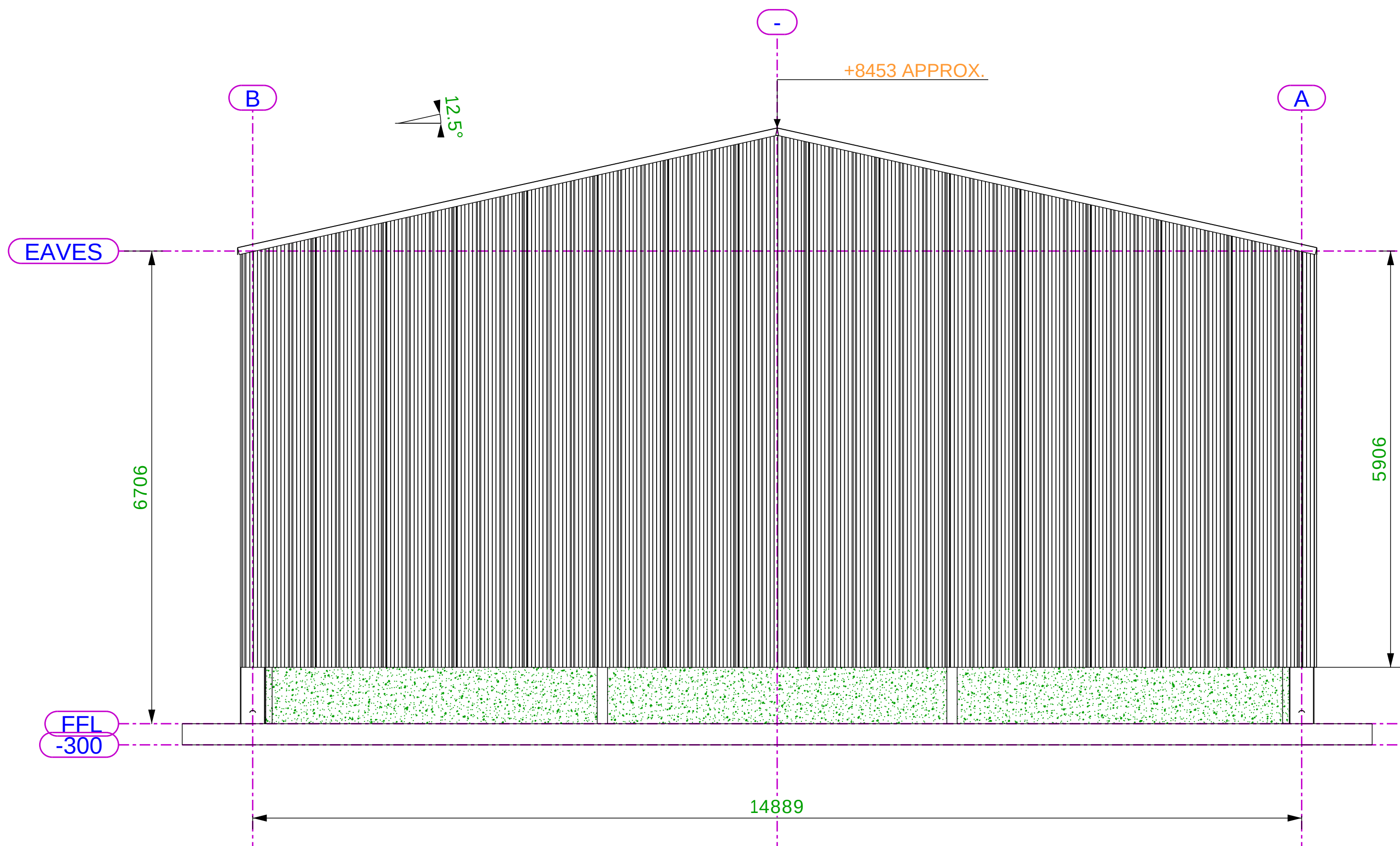
ELEVATION ON GRIDLINE 6
