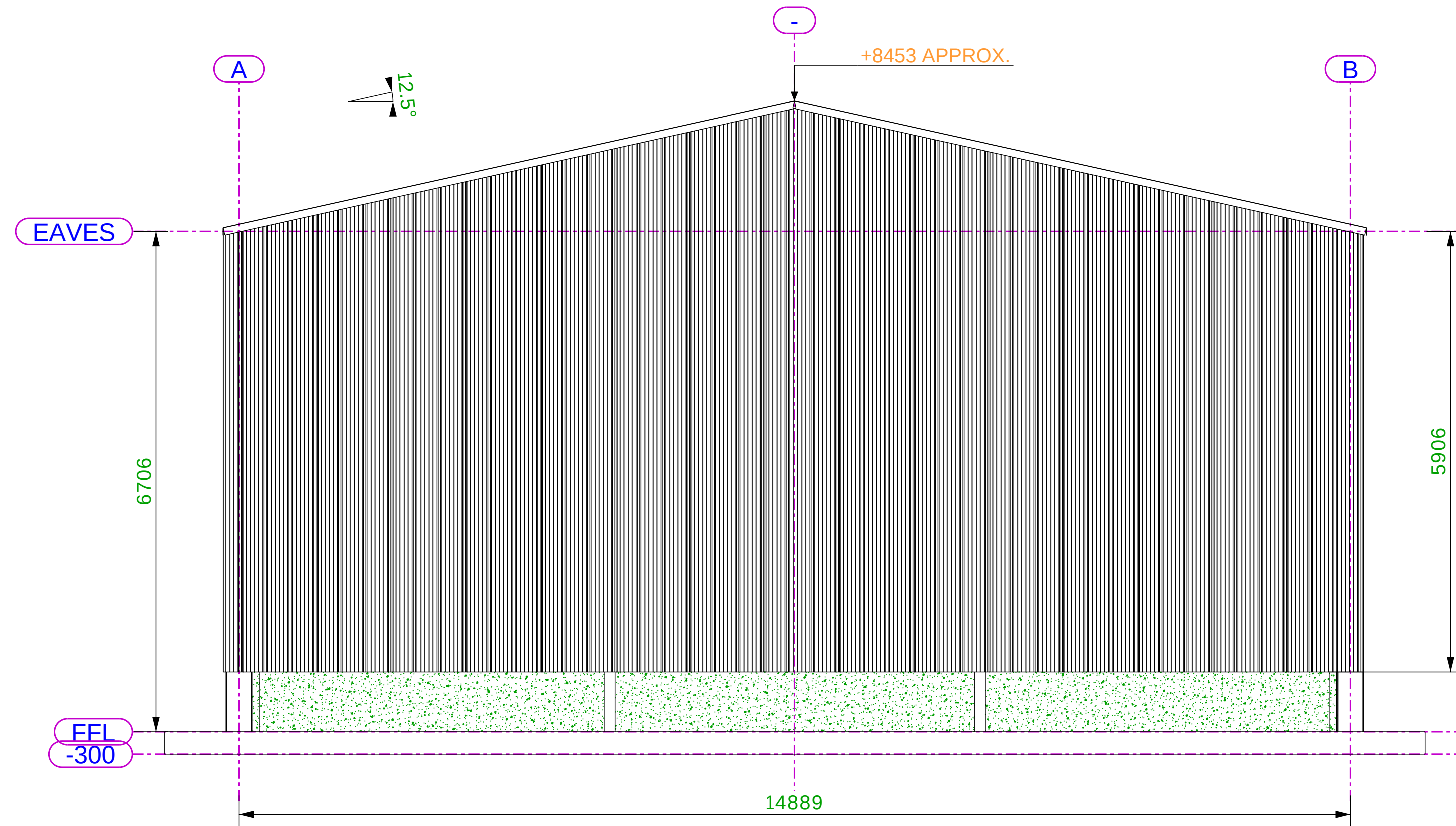
ELEVATION ON GRIDLINE 1
