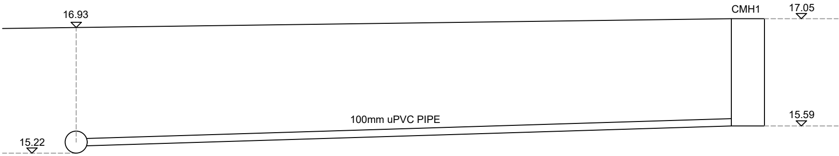
DRAINAGE CONNECTION LONG SECTION Scale 1:50
