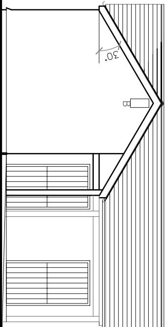
side elevation (sw)
