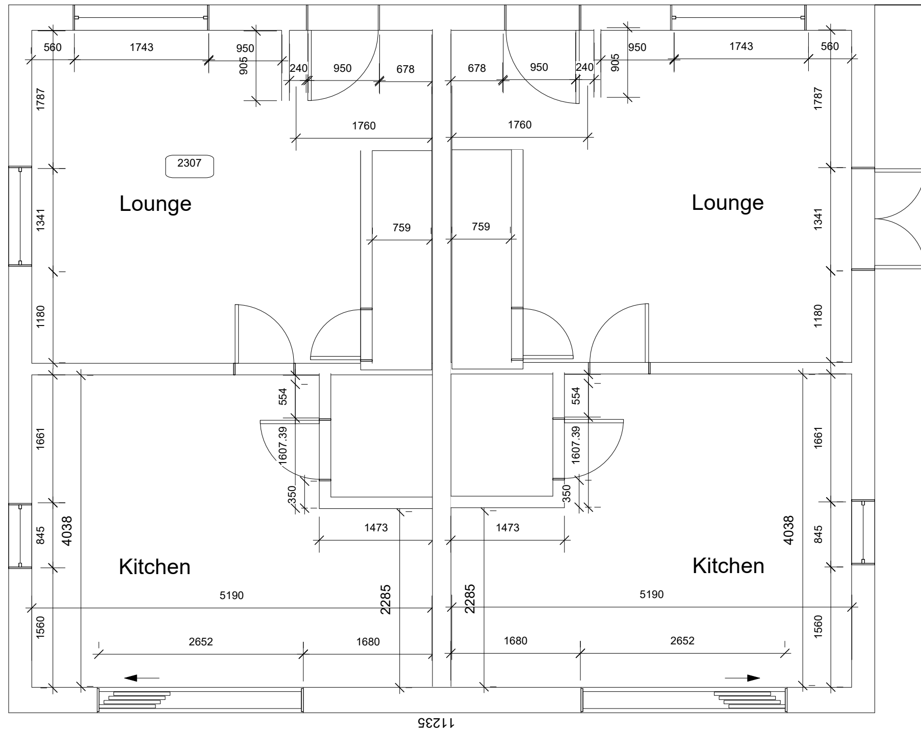
Ground Floor
