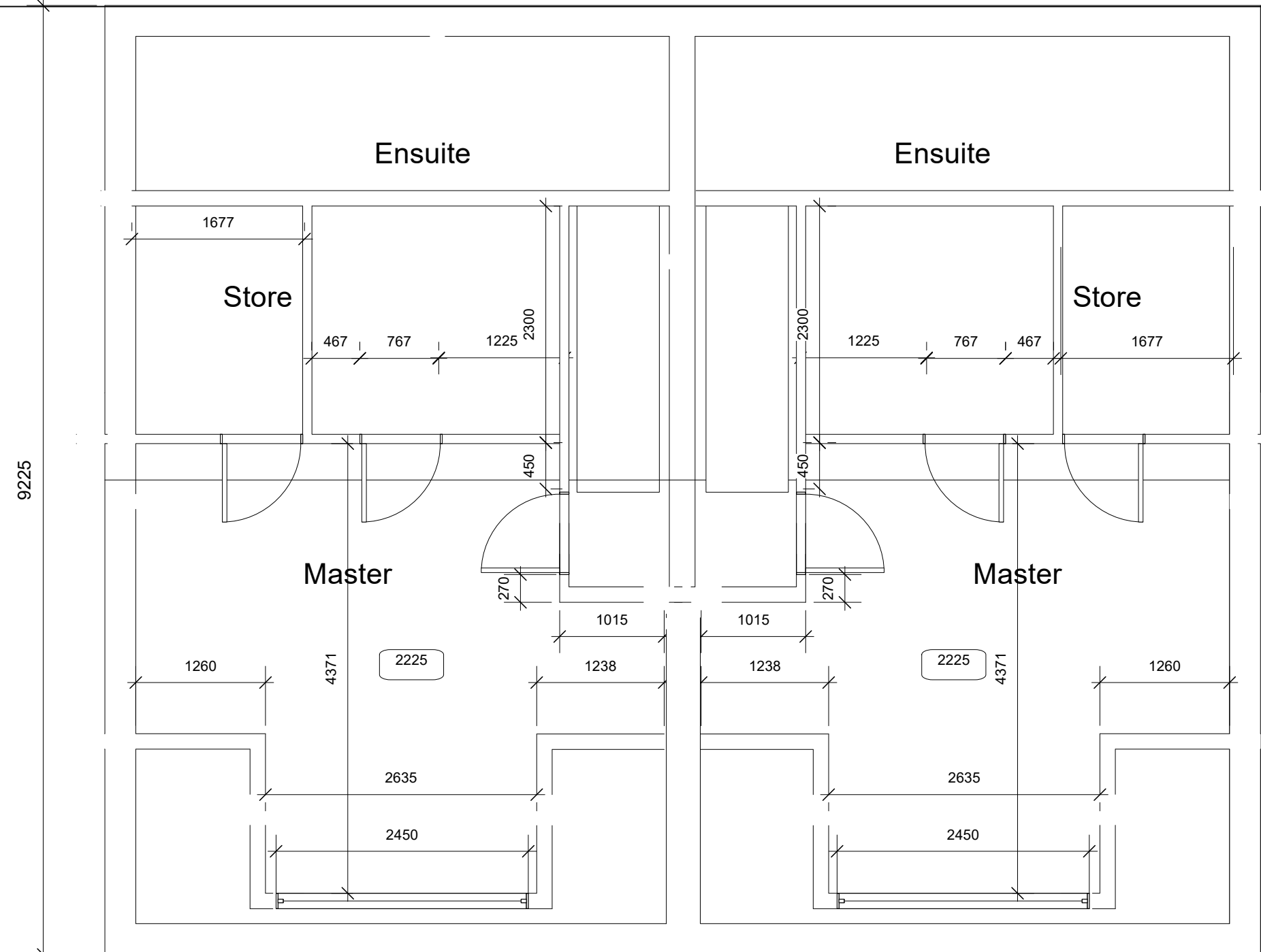
Second Floor
