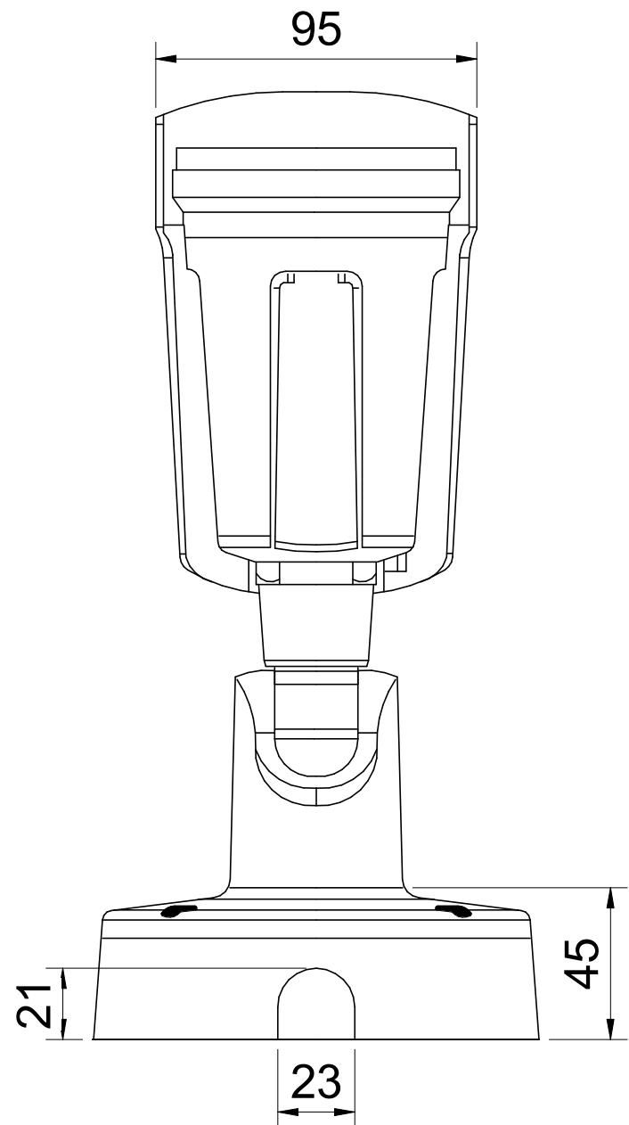
ANPR Camera Top Elevation 1 : 2
