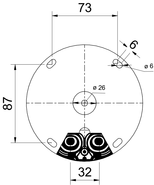
ANPR Camera Back/Fixing Elevation 1 : 2
