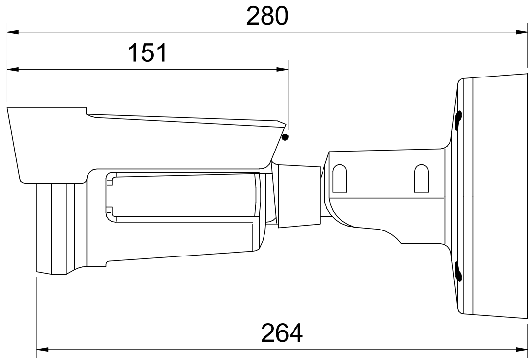
ANPR Camera Side Elevation 1 : 2
