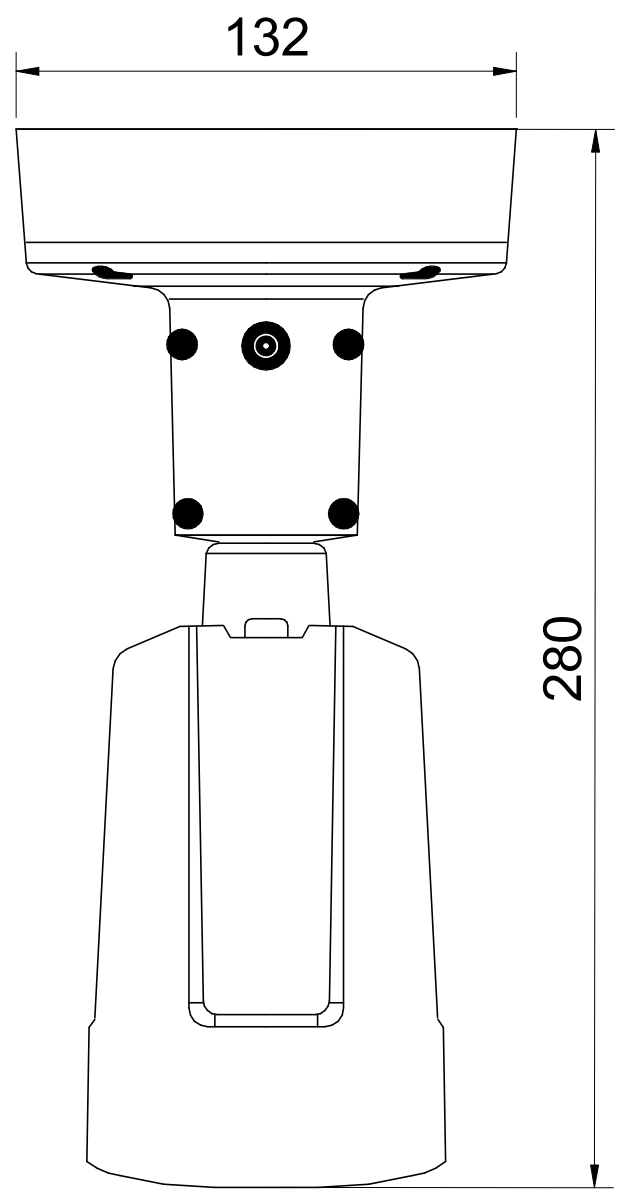
ANPR Camera Bottom Elevation 1 : 2
