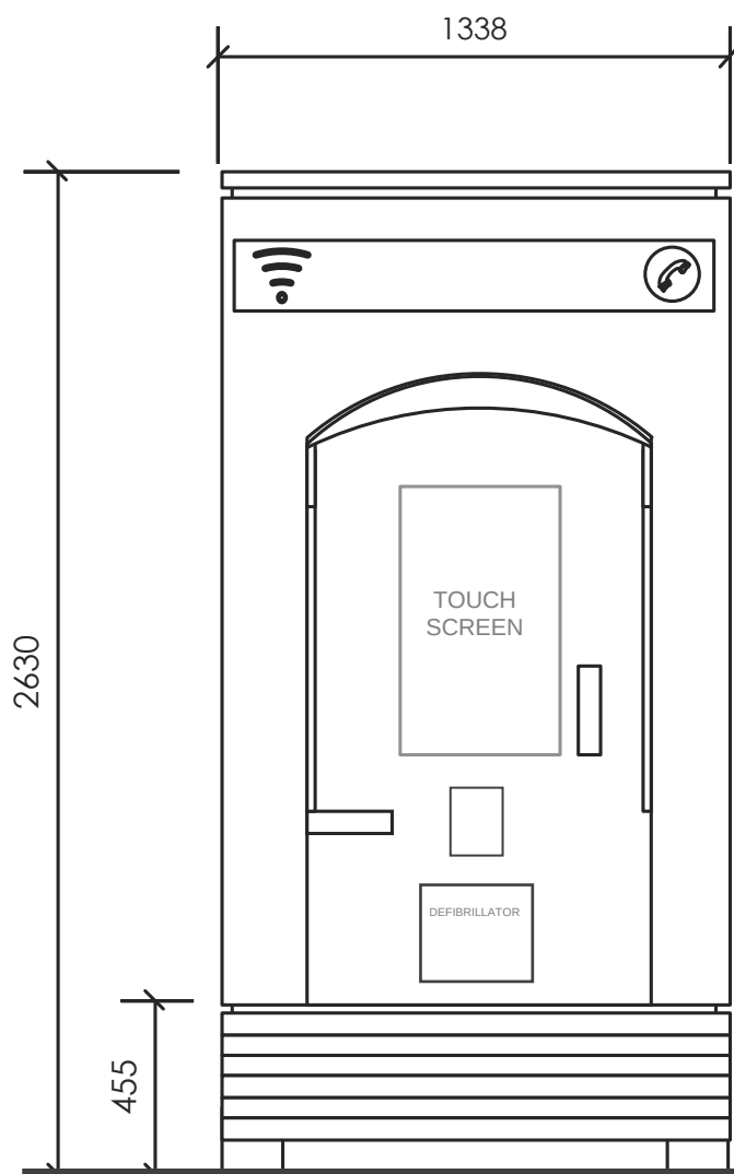
Unit Front
