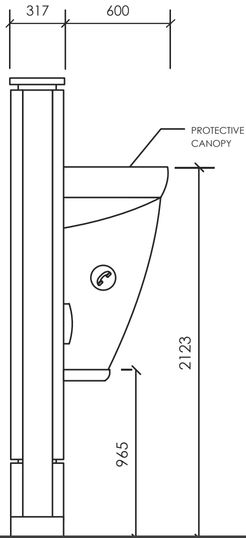
Side
