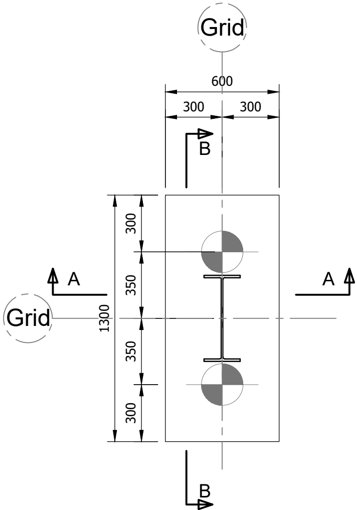
Pile Cap Type 1a (14no. required) Scale 1 : 20
