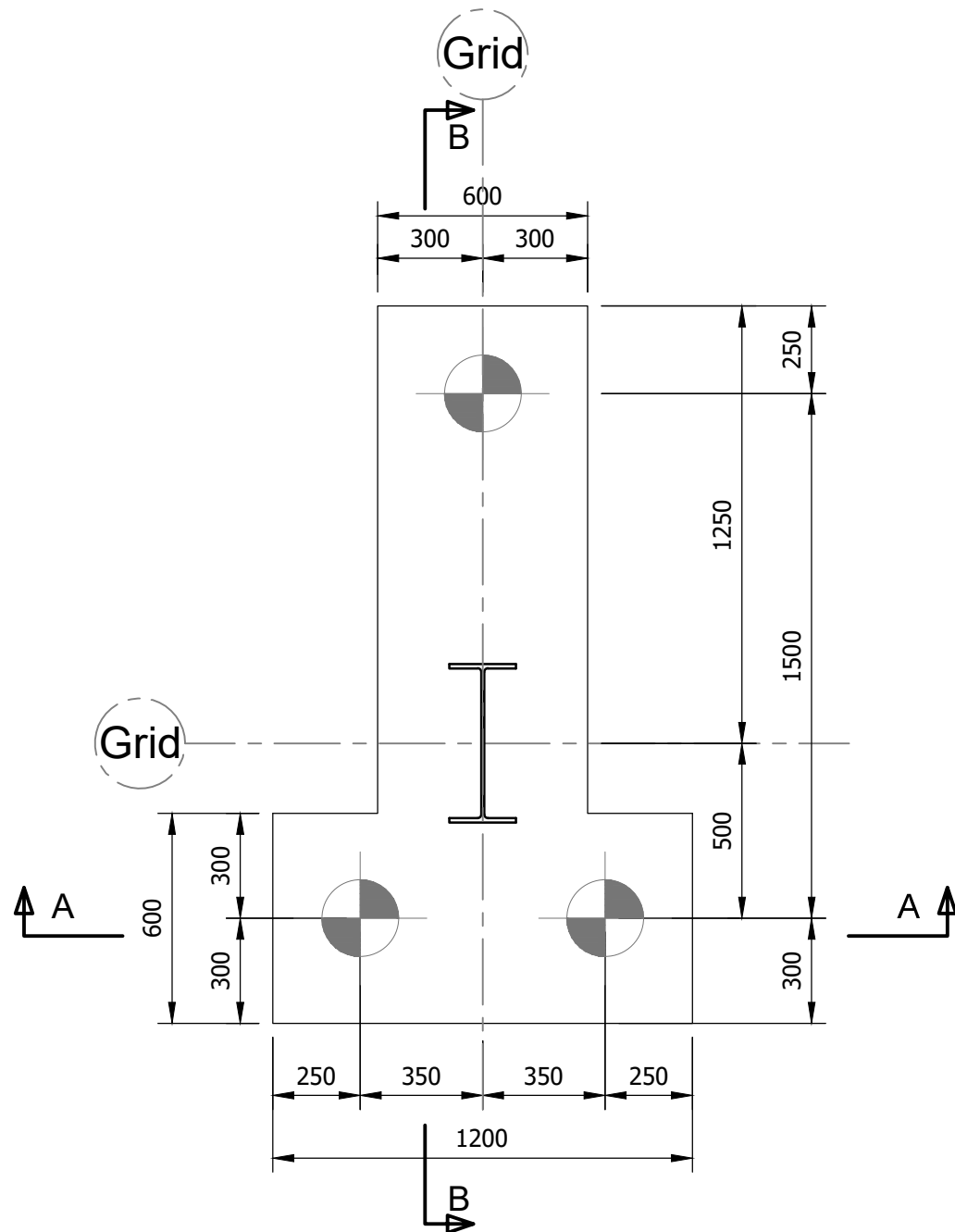
Pile Cap Type 2a (22 no Required) Scale 1 : 20
