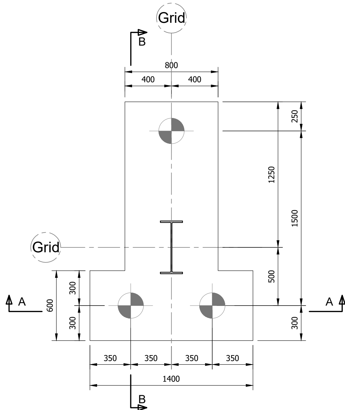
Pile Cap Type 2b (2 no Required) Scale 1 : 20
