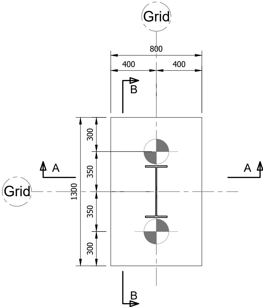
Pile Cap Type 1b (2no. required) Scale 1 : 20
