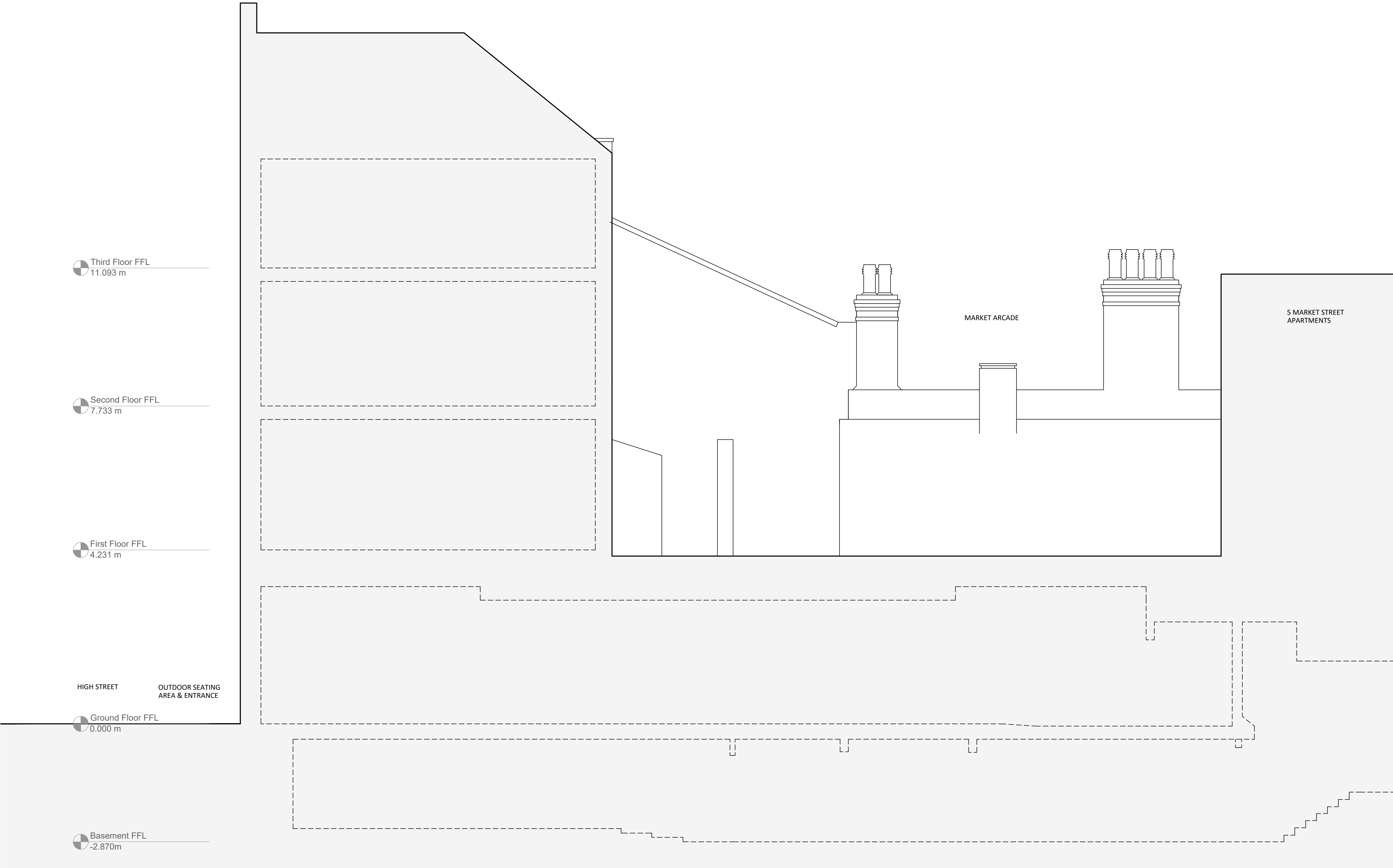
Existing Elevation D 1:50
