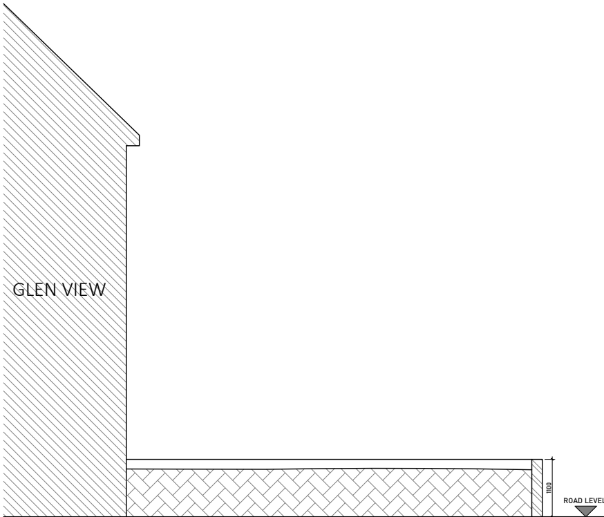
EXISTING SECTION 1:100
