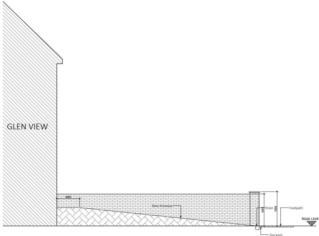
PROPOSED SECTION 1:100
