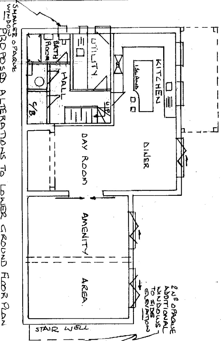
PROPOSED ALTERATIONS TO GROUND FLOOR PLAN
