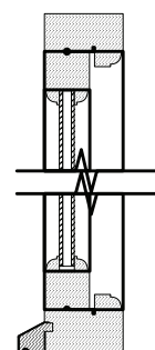
Vertical window section W4
