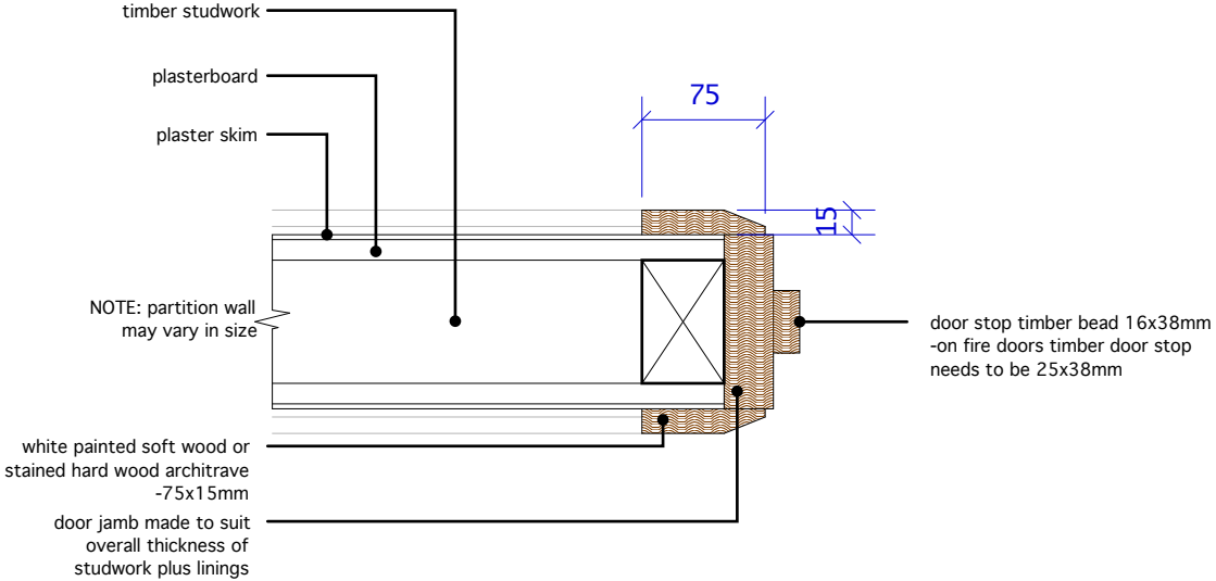
INTERNAL DOOR FRAME DETAIL
