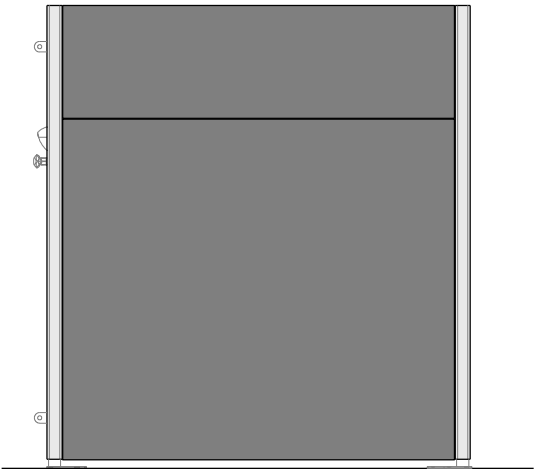
Side Elevations
