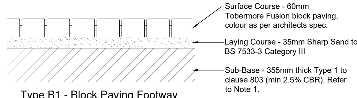
Type B1 - Block Paving Footway No construction trafficking; Occasional heavy traffic loading only; Min 2.5% CBR
