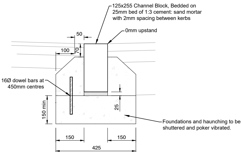
Kerbing Type CS - 125x255mm CS1 Channel Block
