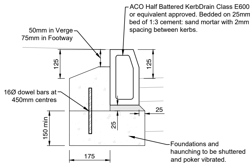
Kerbing Type KD - ACO Kerbdrain E600
