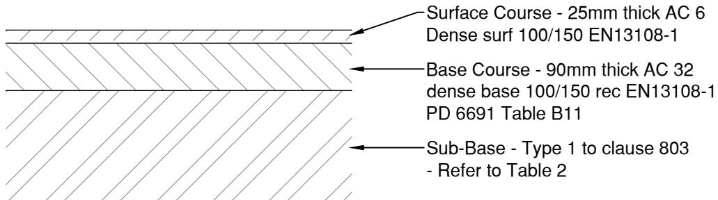
Type F1 - Footway (Where significant HGV overrun is likely)
