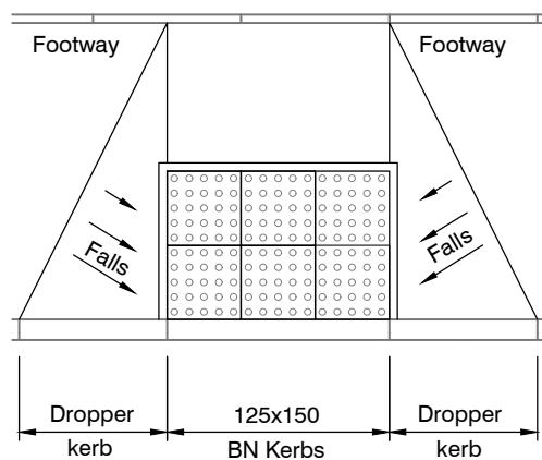
Tactile Paving Crossing Detail
