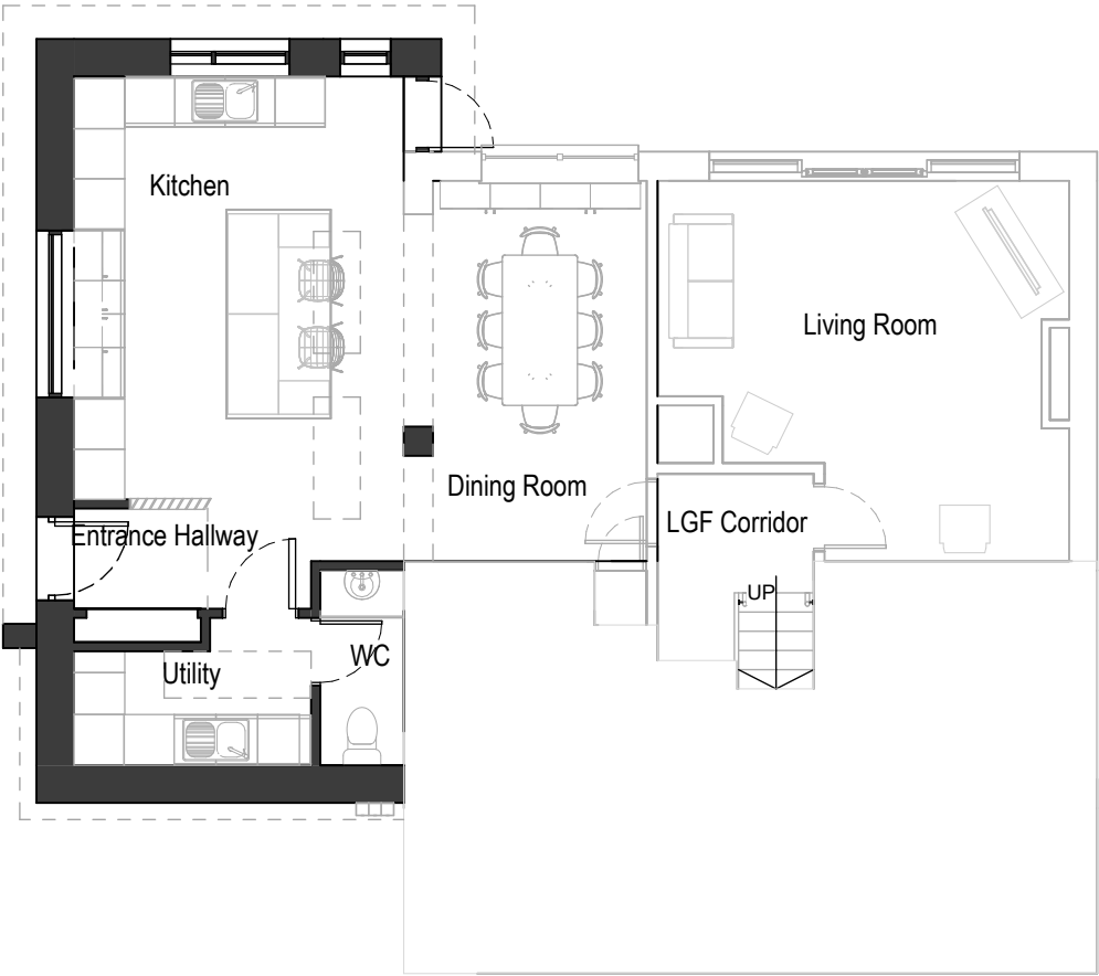
Proposed Lower Ground Floor 1 : 100
