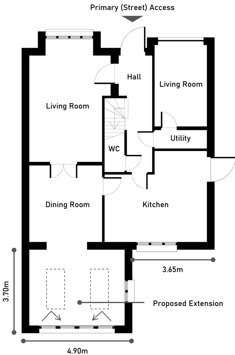
PROPOSED GROUND FLOOR PLAN GA
