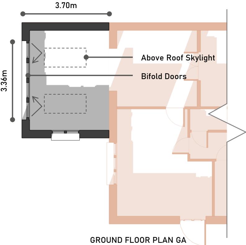
GROUND FLOOR PLAN GA
