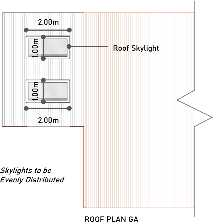
ROOF PLAN GA
