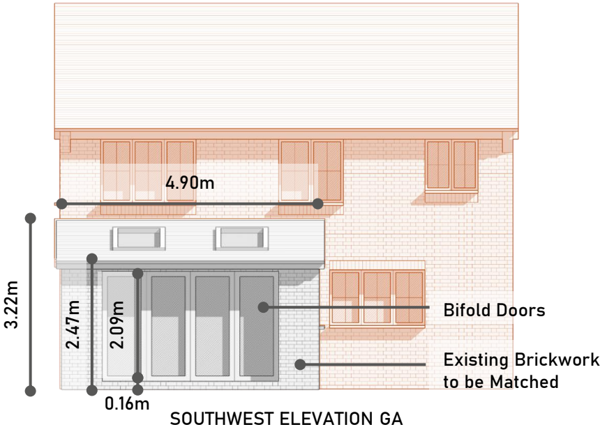
SOUTHWEST ELEVATION GA
