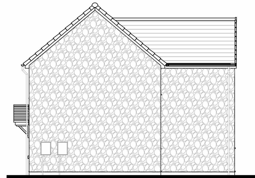
SIDE B ELEVATION
