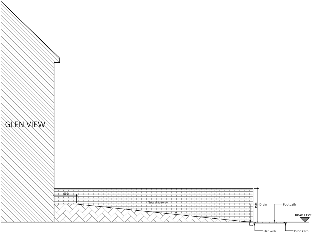
PROPOSED SECTION 1:100
