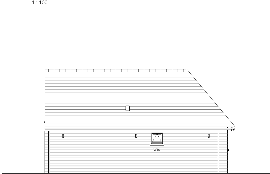
Proposed Elevation 05 1 : 100
