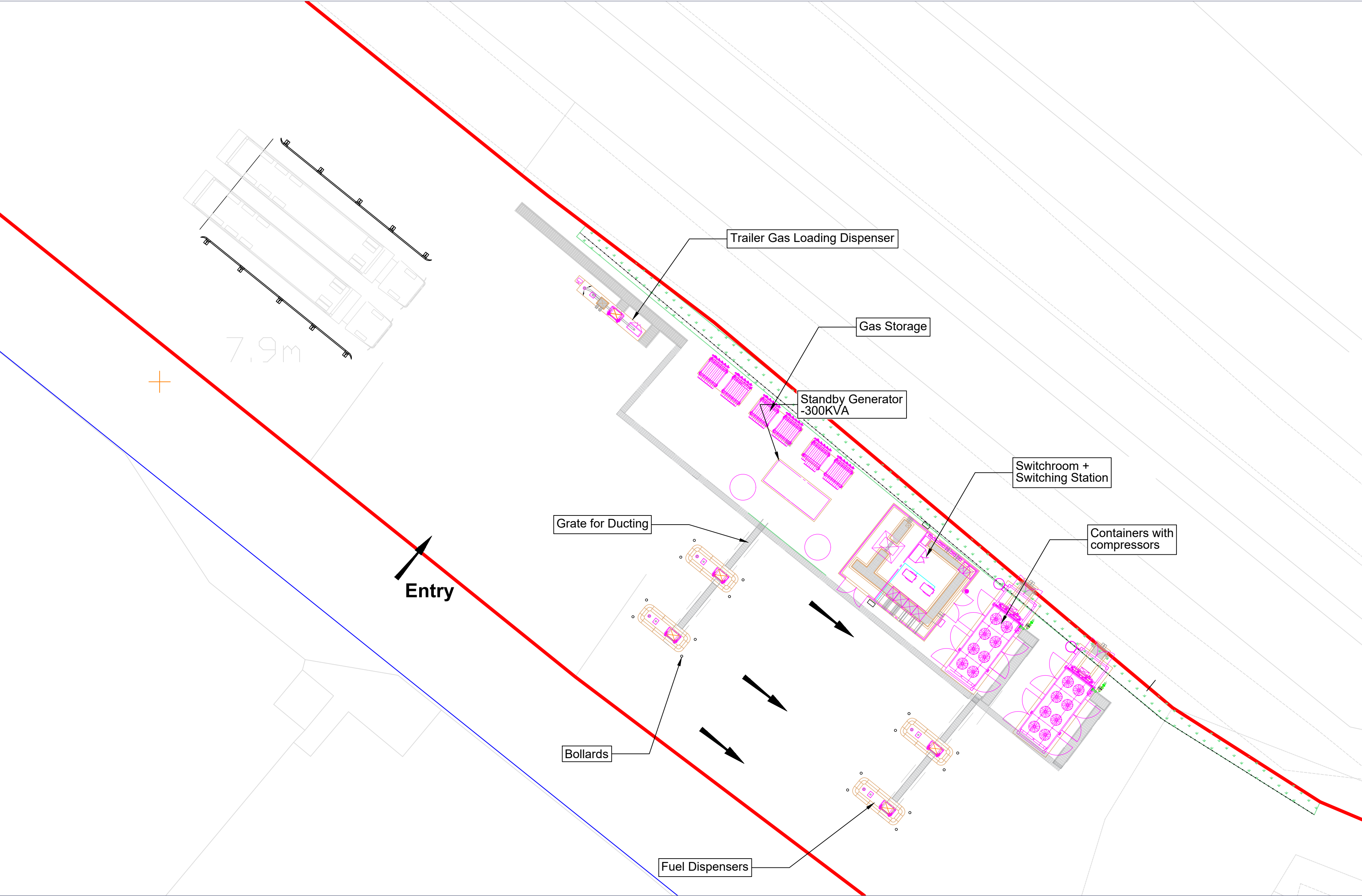
Proposed Site Layout Scale (1:200)
