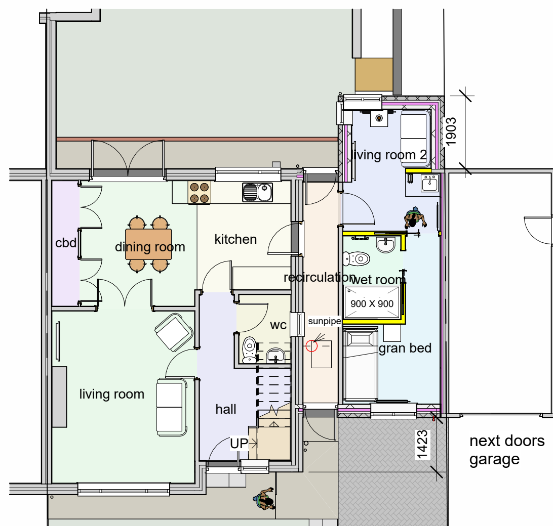
8 0_grd FFL Proposed 1 : 100
