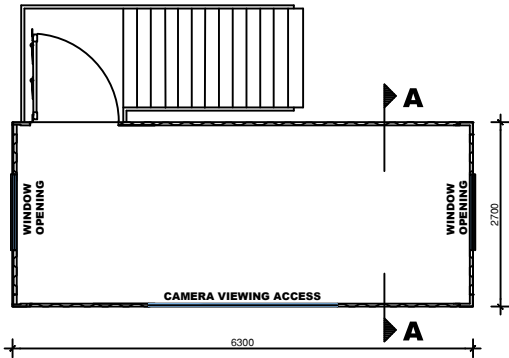
TOP CONTAINER PLAN
